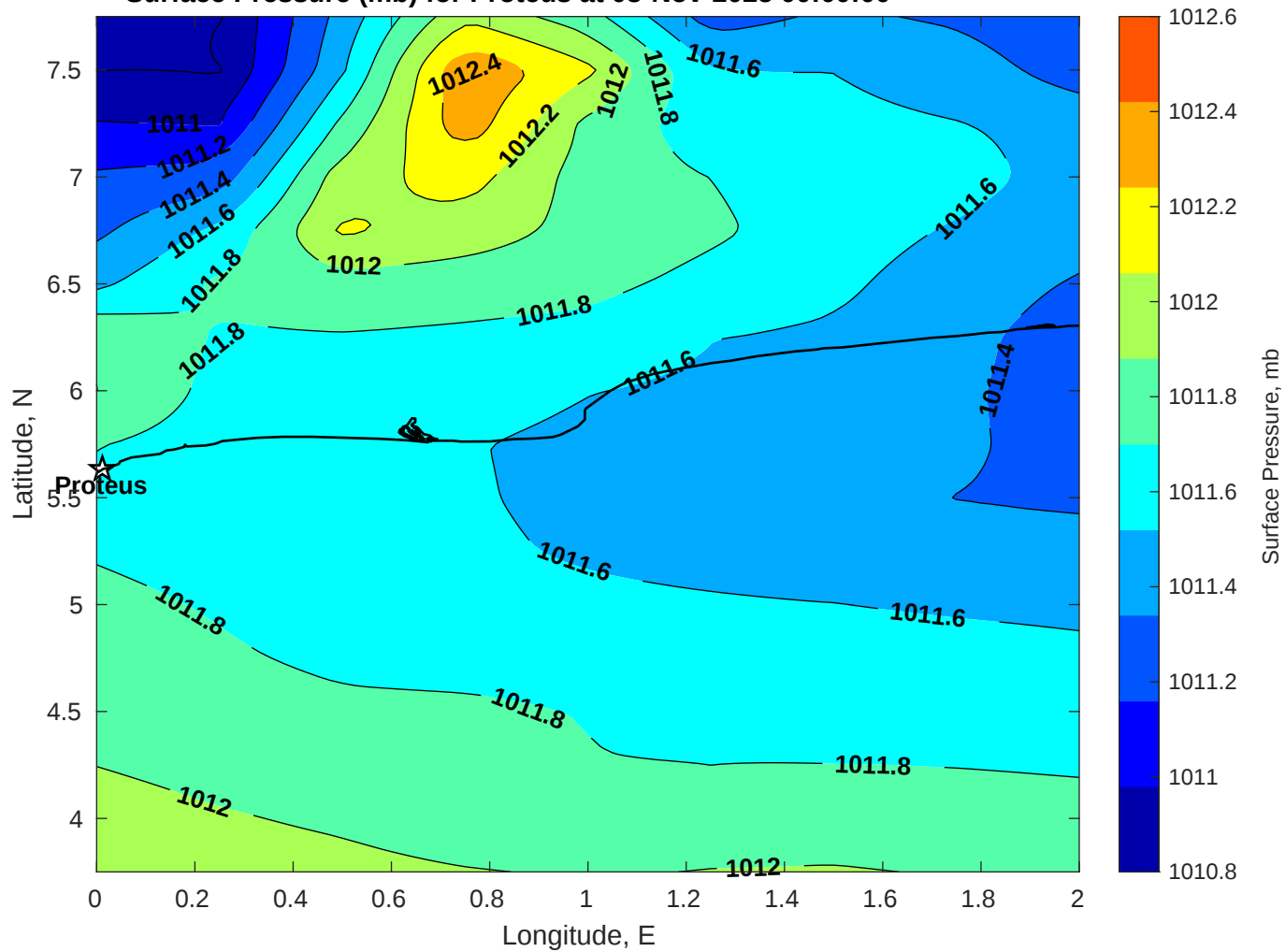
Surface Pressure (mb) for Proteus at 03-Nov-2025 00:00:00
