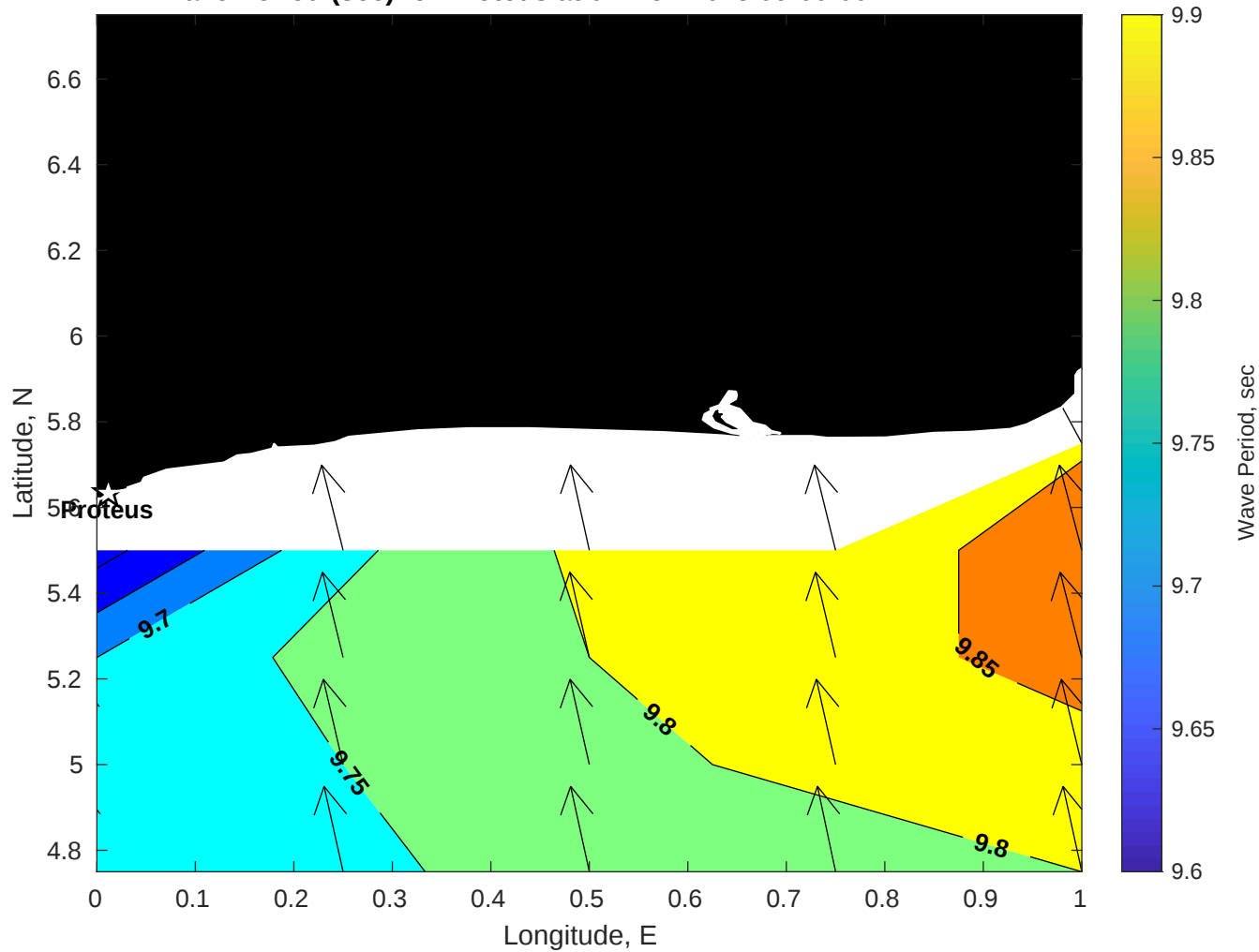
Wave Period (sec) for Proteus at 02-Nov-2025 09:00:00
