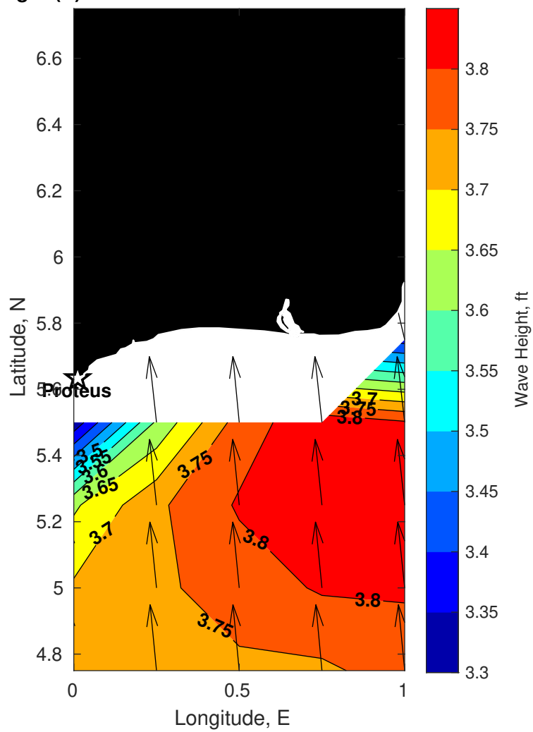
Wave Height (ft) for Proteus at 02-Nov-2025 09:00:00
