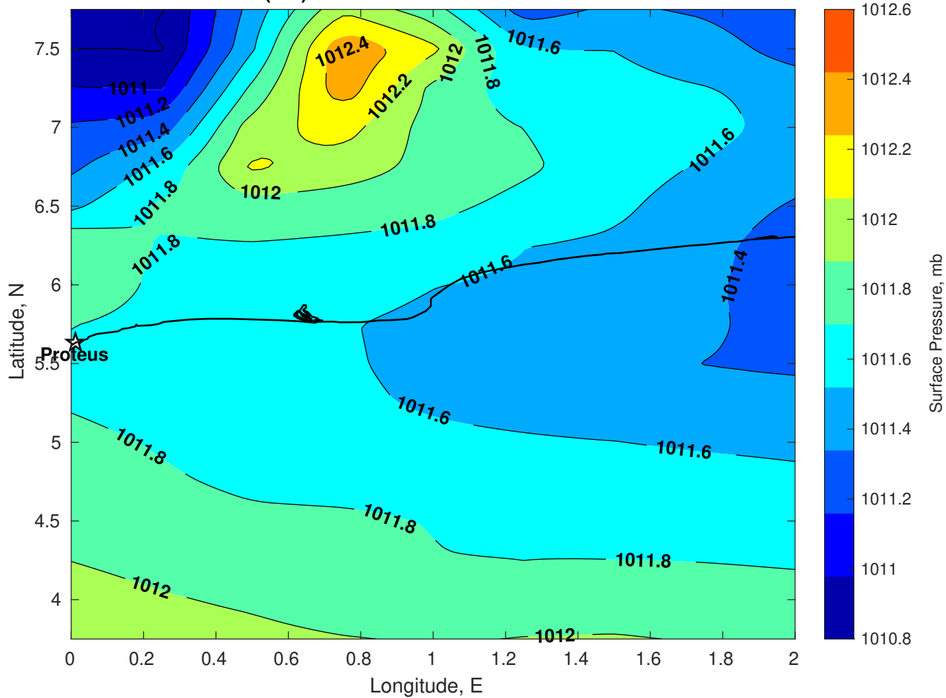
Surface Pressure (mb) for Proteus at 03-Nov-2025 00:00:00
