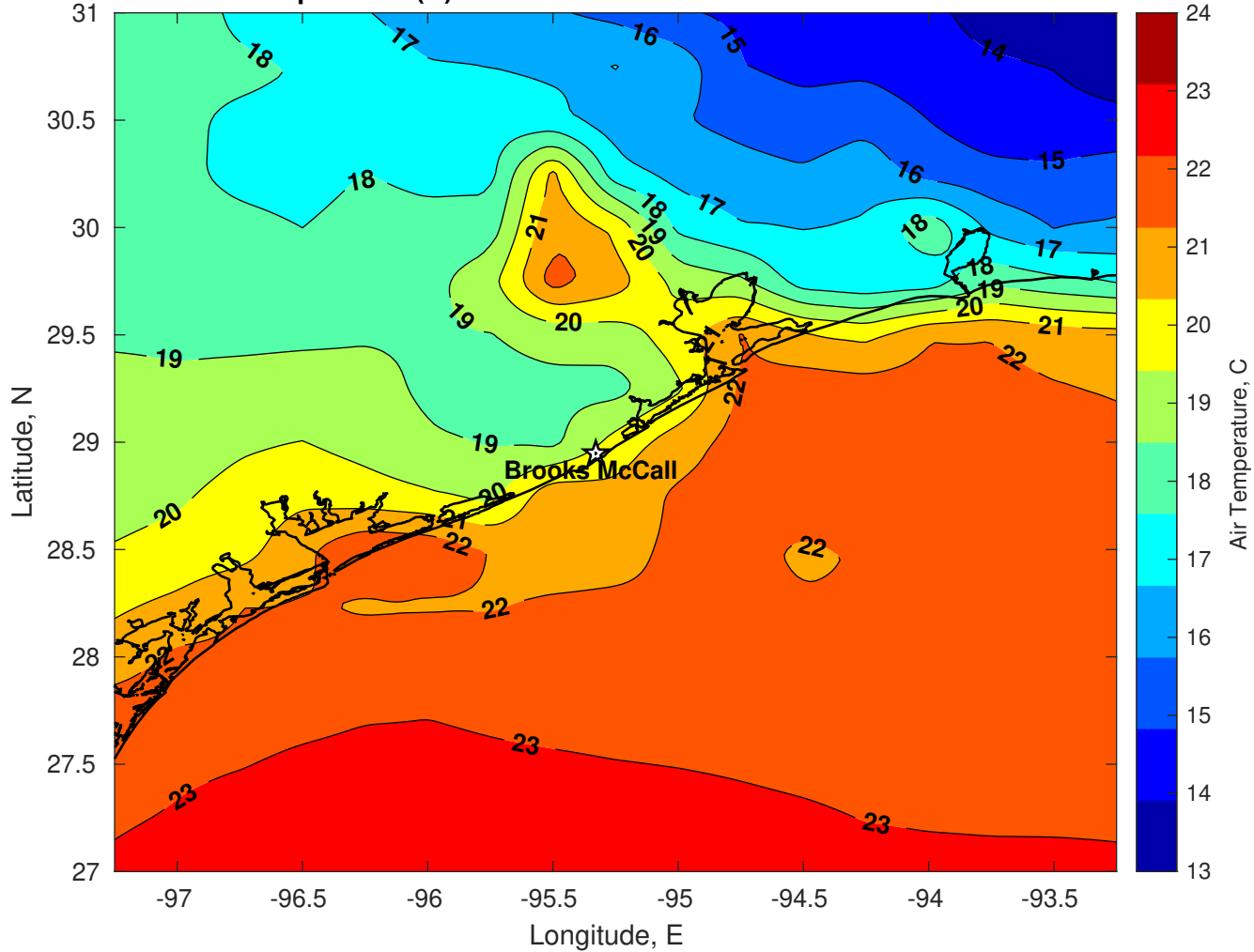
Air Temperature (C) for Brooks McCall at 03-Nov-2025
