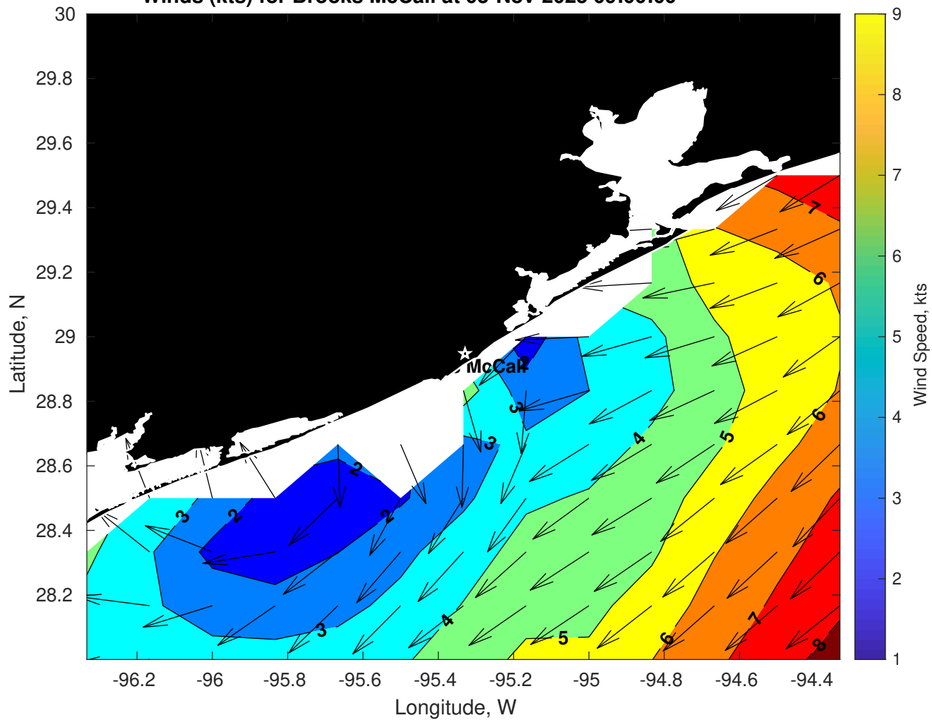
Winds (kts) for Brooks McCall at 03-Nov-2025 09:00:00
