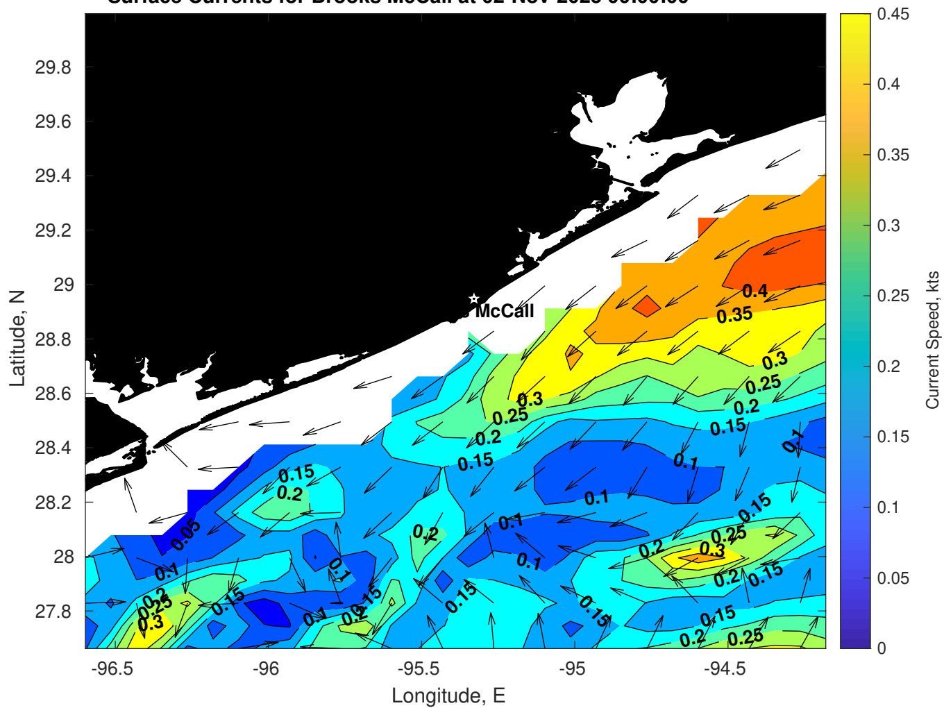
Surface Currents for Brooks McCall at 02-Nov-2025 00:00:00
