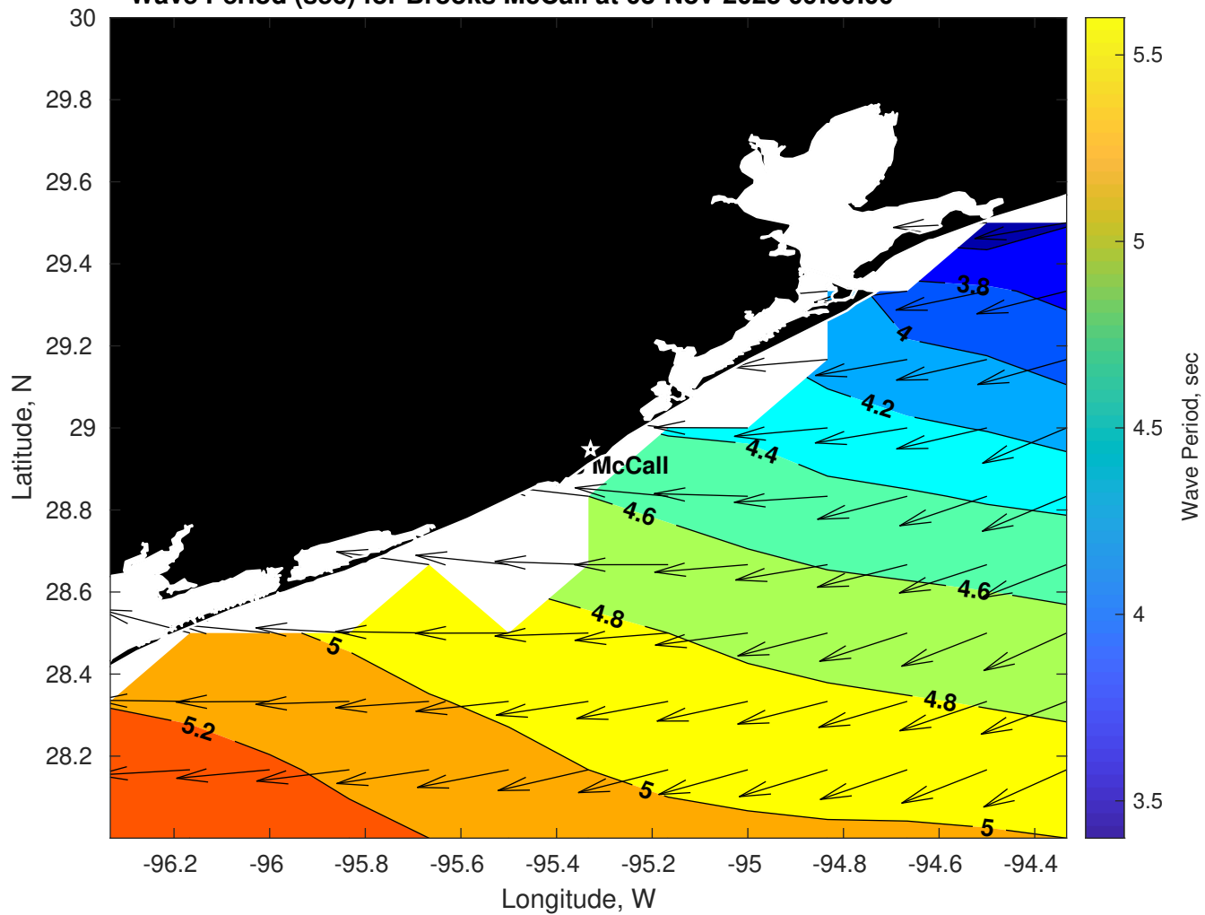
Wave Period (sec) for Brooks McCall at 03-Nov-2025 09:00:00
