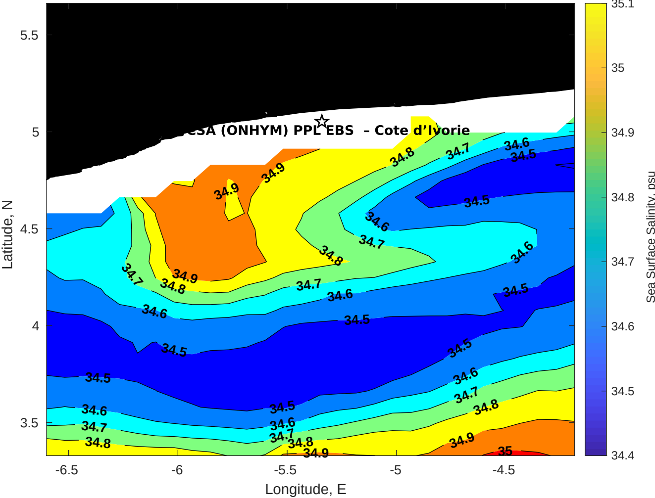
Surface Salinity for CSA (ONHYM) PPL EBS - Cote d'Ivoire at 02-Nov-2025 00:00:00
