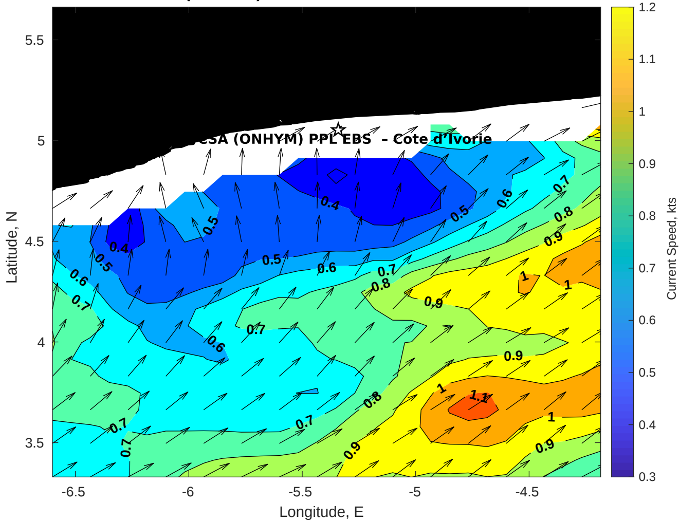
Surface Currents for CSA (ONHYM) PPL EBS - Cote d'Ivoire at 02-Nov-2025 00:00:00
