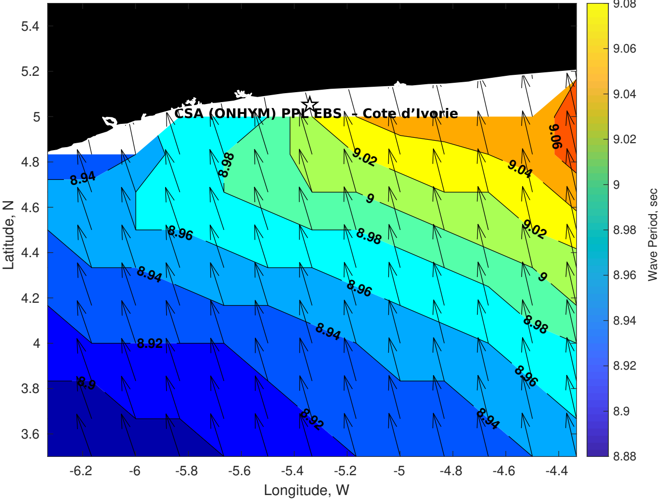
Wave Period (sec) for CSA (ONHYM) PPL EBS - Cote d'Ivoire at 03-Nov-2025 09:00:00
