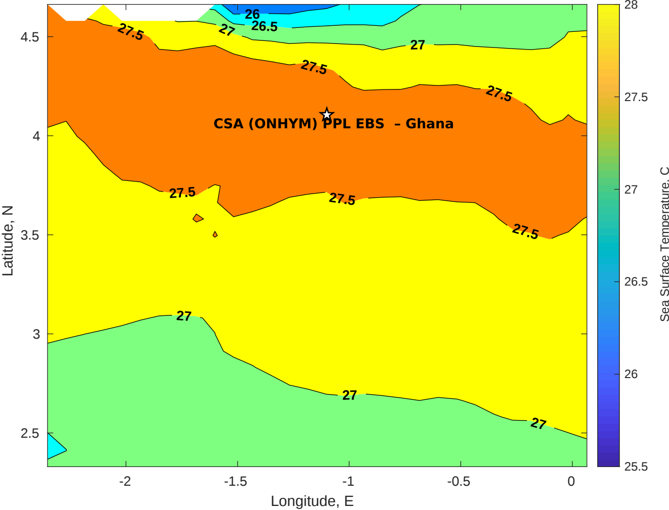
SST for CSA (ONHYM) PPL EBS - Ghana at 02-Nov-2025 00:00:00
