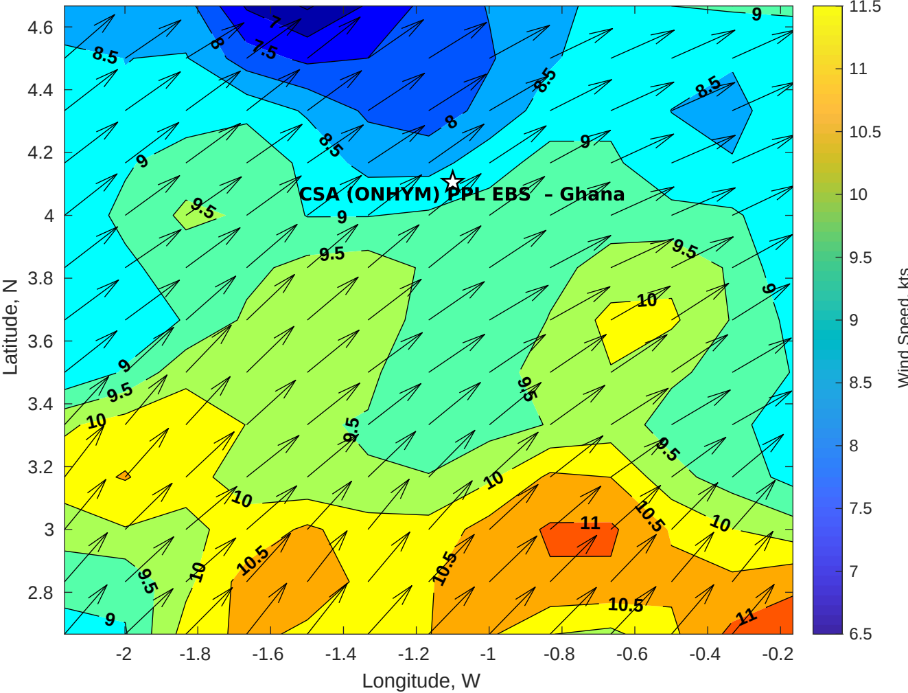
Winds (kts) for CSA (ONHYM) PPL EBS - Ghana at 03-Nov-2025 09:00:00
