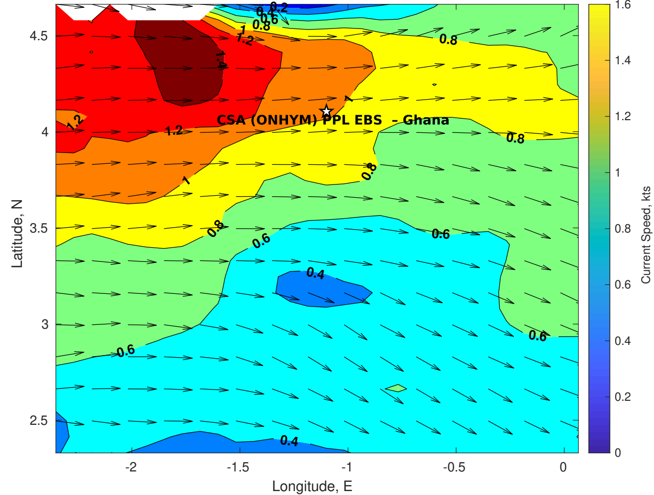
Surface Currents for CSA (ONHYM) PPL EBS - Ghana at 02-Nov-2025 00:00:00
