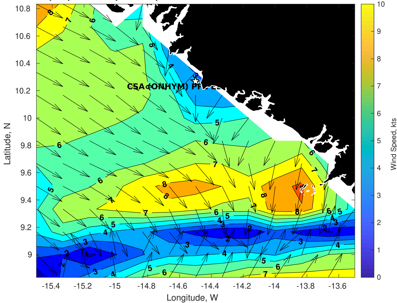
Winds (kts) for CSA (ONHYM) PPL EBS - Guinea at 03-Nov-2025 09:00:00
