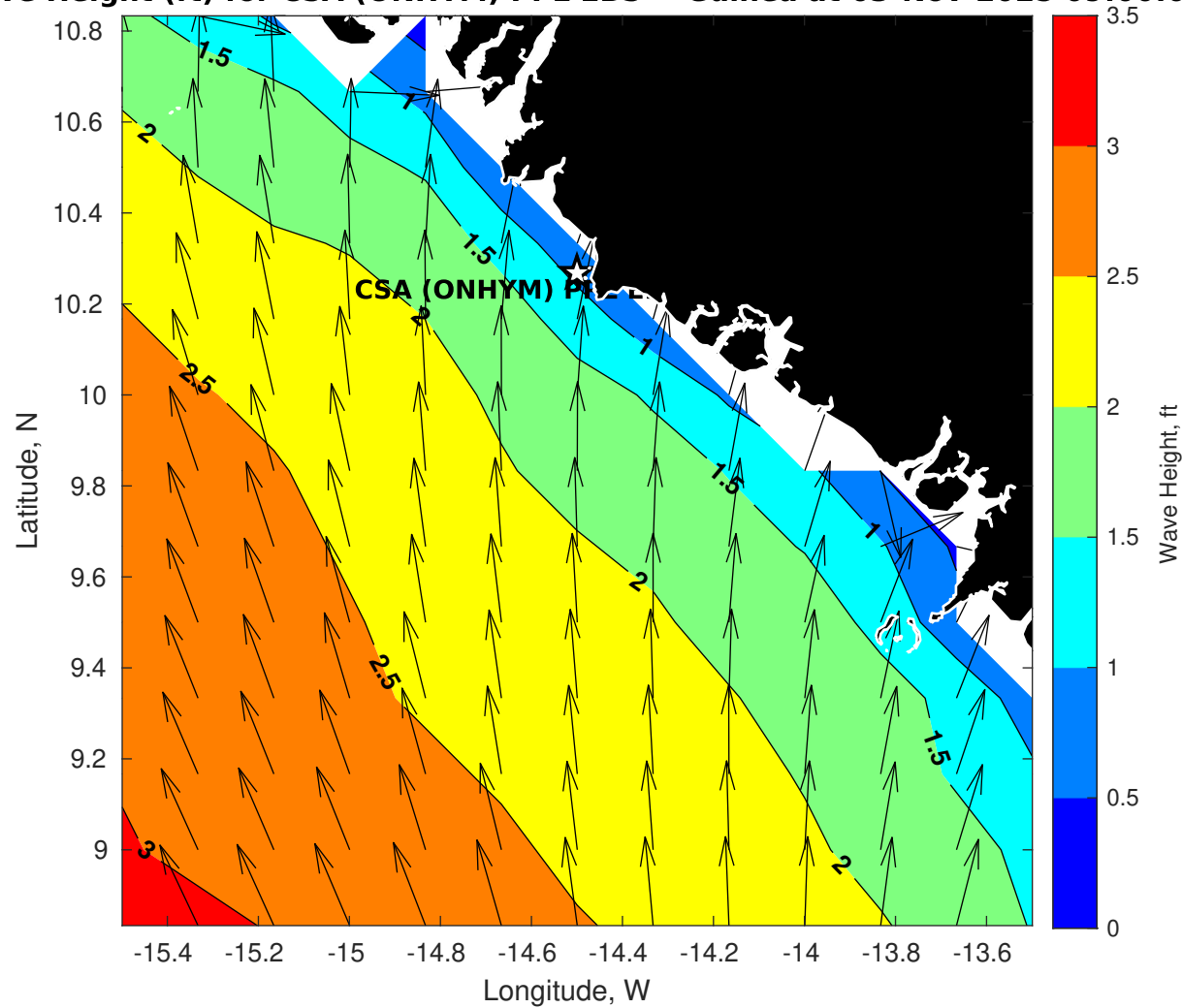
Wave Height (ft) for CSA (ONHYM) PPL EBS - Guinea at 03-Nov-2025 09:00:00
