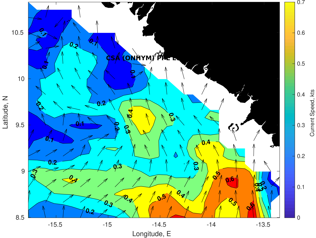
Surface Currents for CSA (ONHYM) PPL EBS - Guinea at 02-Nov-2025 00:00:00
