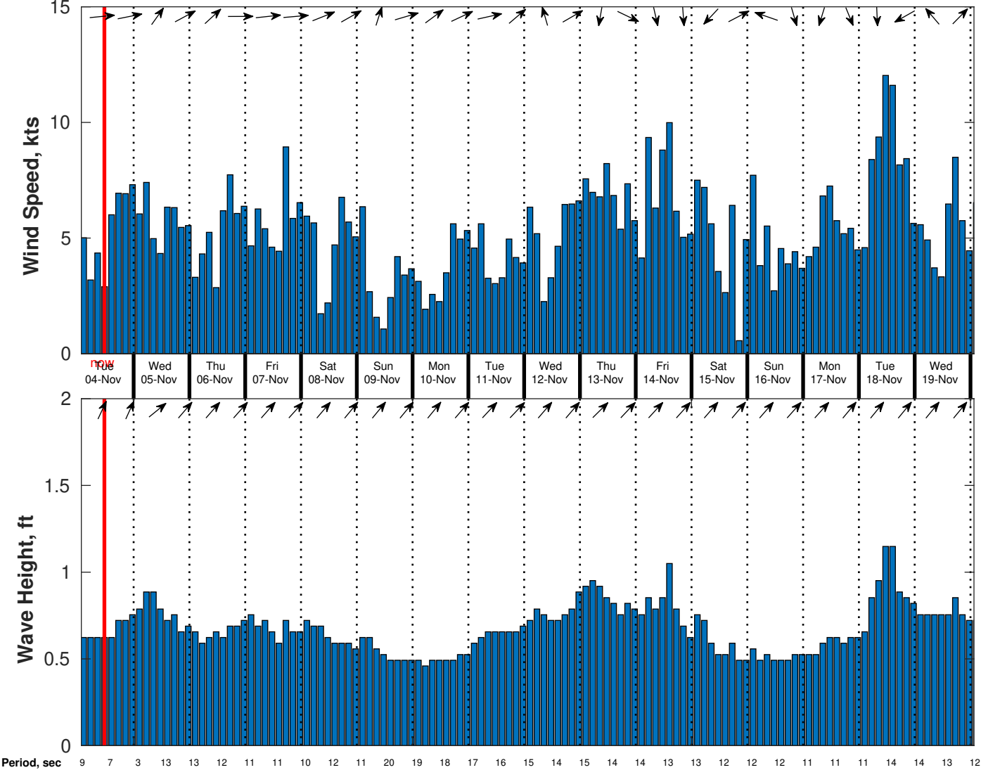
Wind & Wave Forecast for CSA (ONHYM) PPL EBS - Guinea from 03-Nov-2025 01:00:00 to 19-Nov-2025 01:00:00
