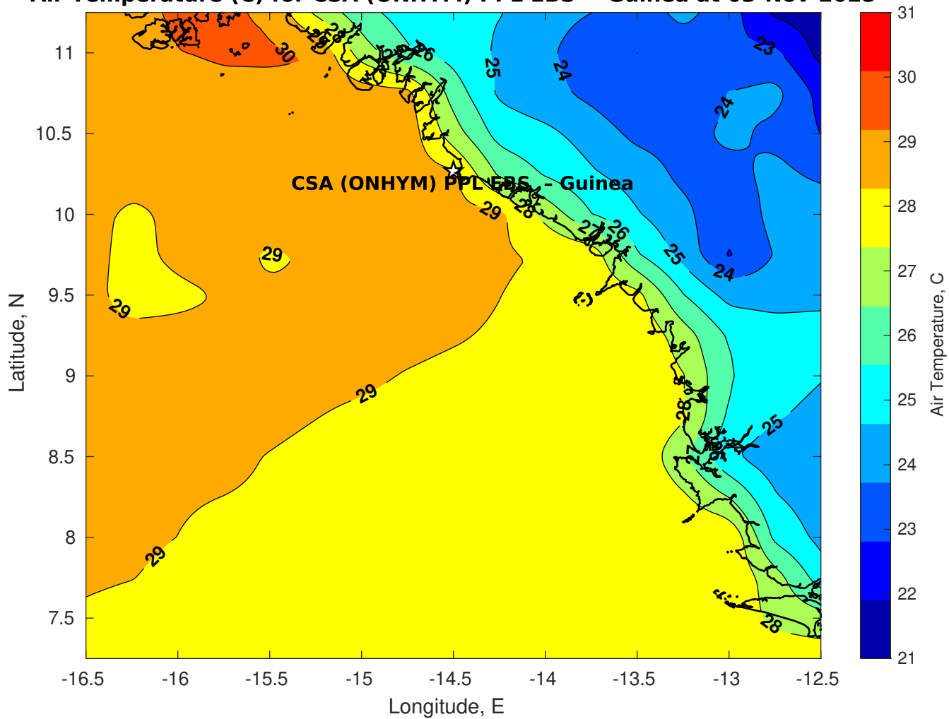
Air Temperature (C) for CSA (ONHYM) PPL EBS - Guinea at 03-Nov-2025
