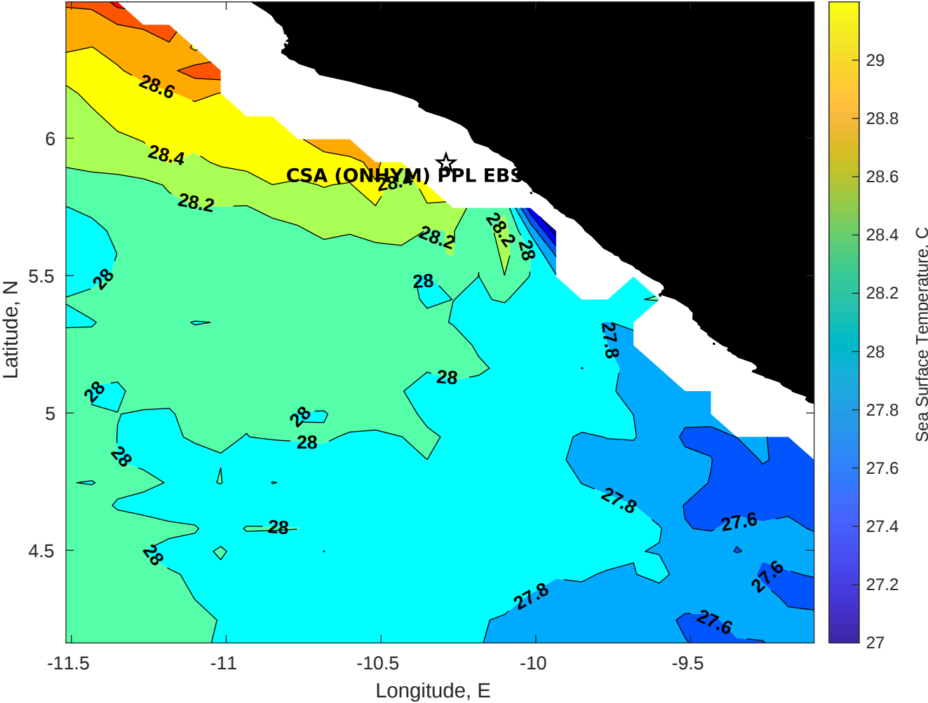
SST for CSA (ONHYM) PPL EBS - Liberia at 02-Nov-2025 00:00:00
