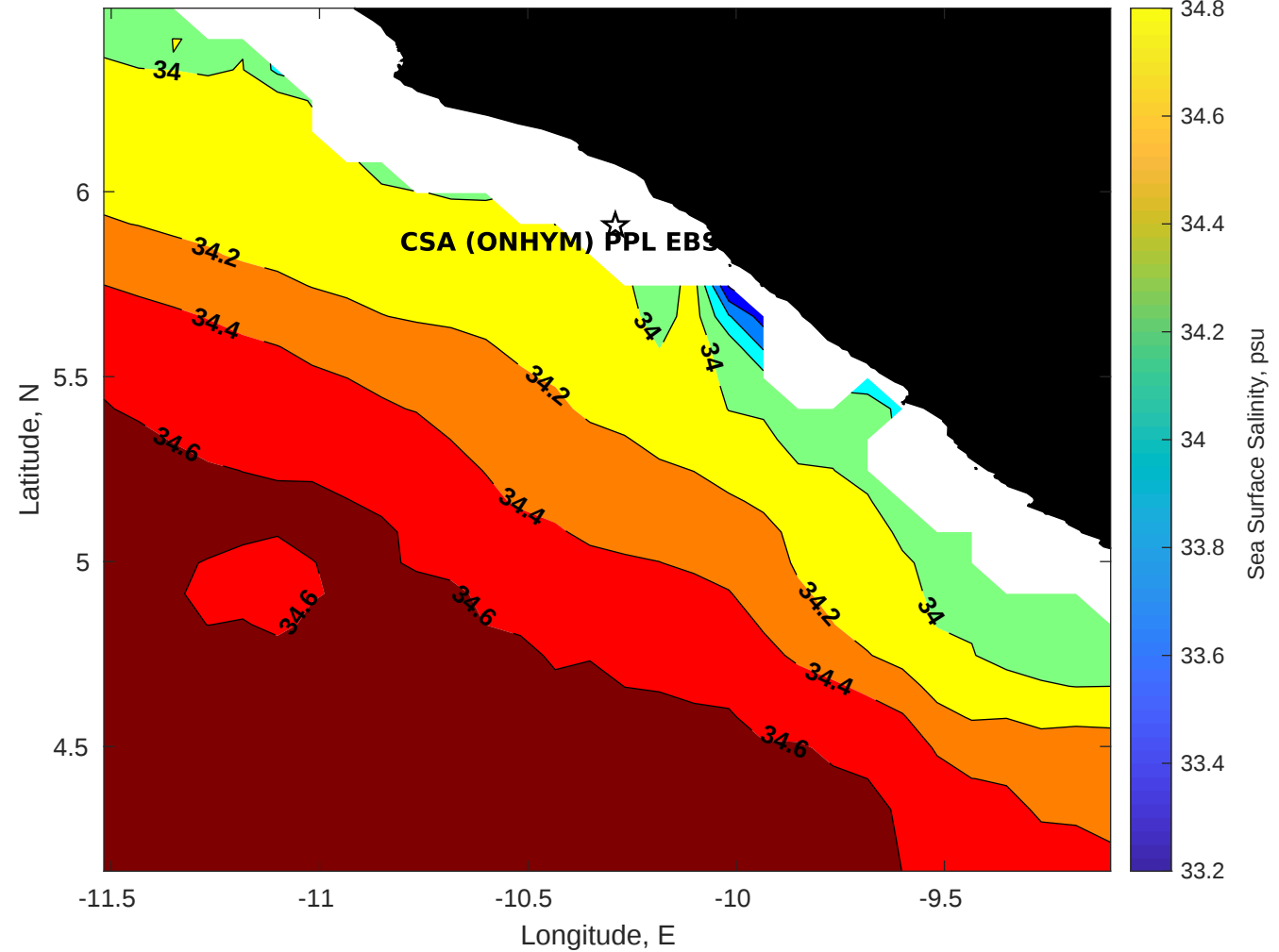
Surface Salinity for CSA (ONHYM) PPL EBS - Liberia at 02-Nov-2025 00:00:00
