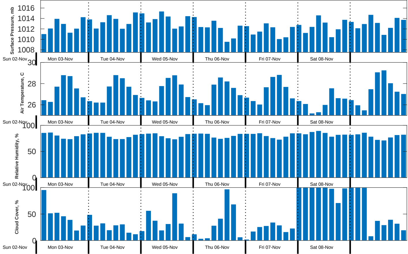
Met Forecast for CSA (ONHYM) PPL EBS - Liberia from 03-Nov-2025 00:00:00 to 10-Nov-2025 00:00:00
