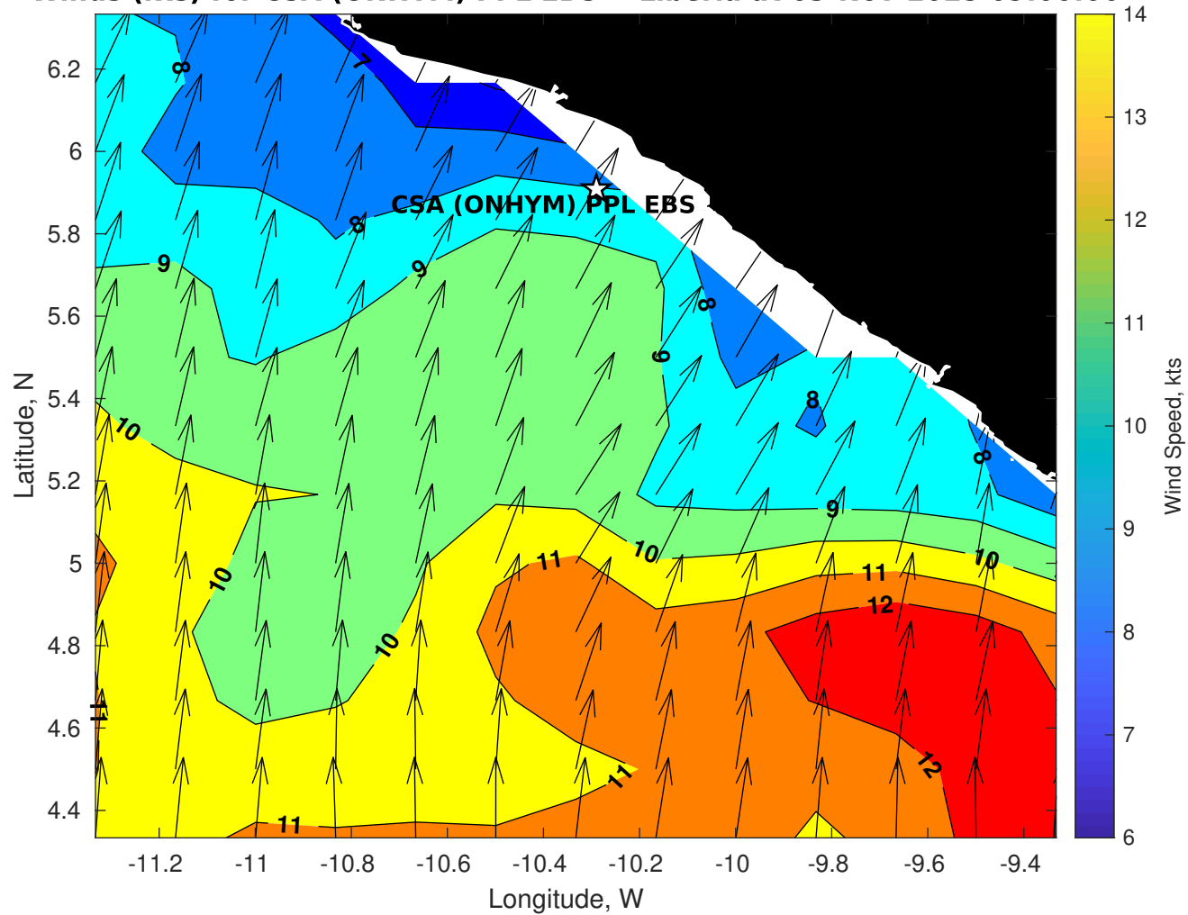
Winds (kts) for CSA (ONHYM) PPL EBS - Liberia at 03-Nov-2025 09:00:00
