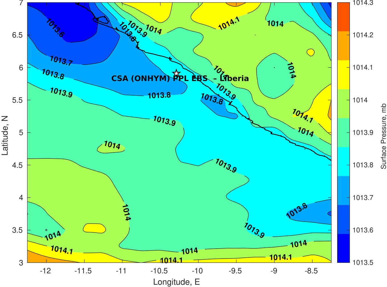
Surface Pressure (mb) for CSA (ONHYM) PPL EBS - Liberia at 04-Nov-2025 00:00:00
