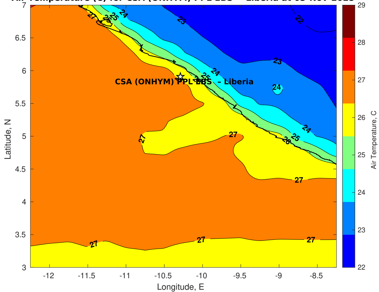
Air Temperature (C) for CSA (ONHYM) PPL EBS - Liberia at 03-Nov-2025
