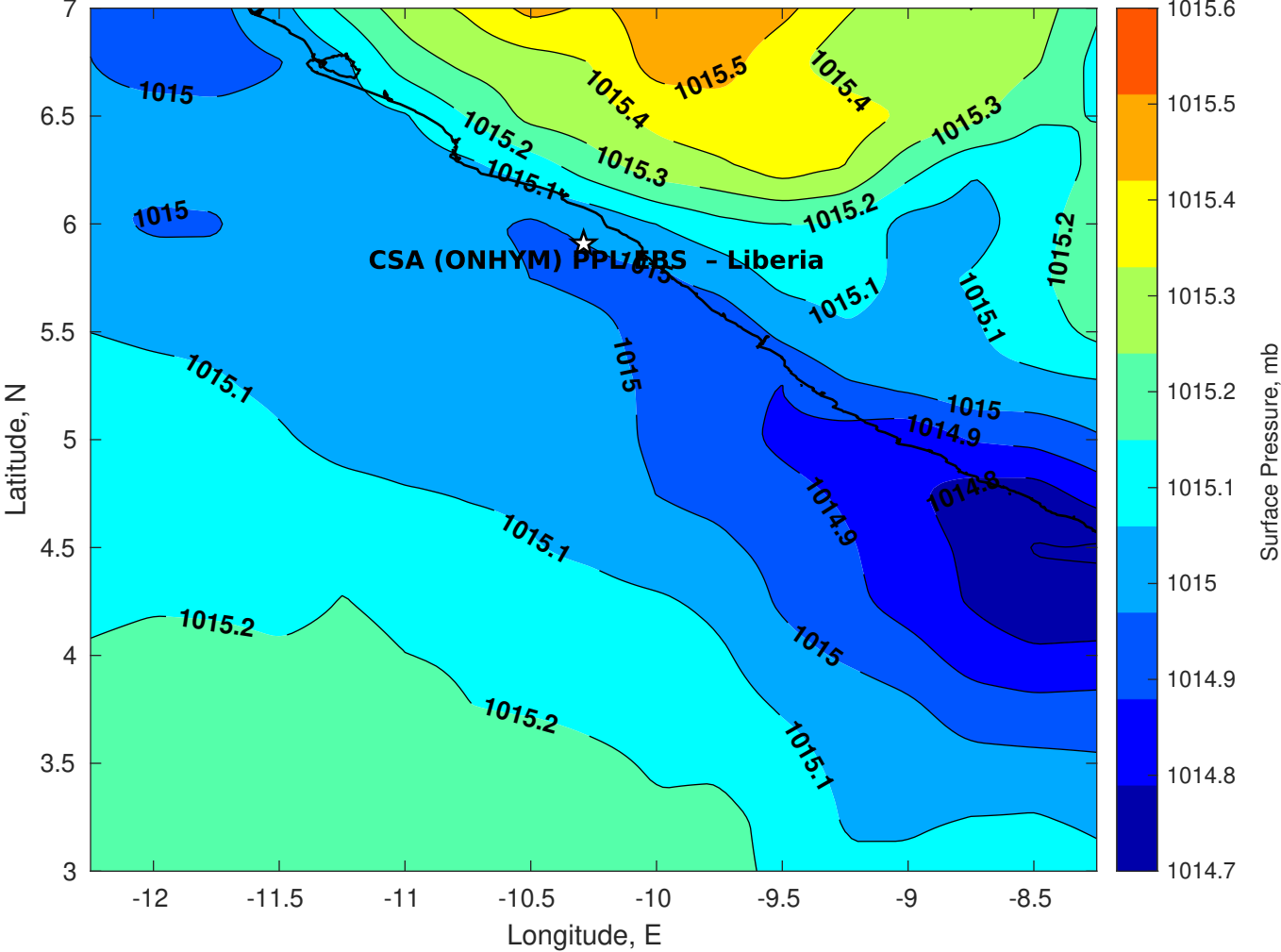
Surface Pressure (mb) for CSA (ONHYM) PPL EBS - Liberia at 05-Nov-2025 00:00:00
