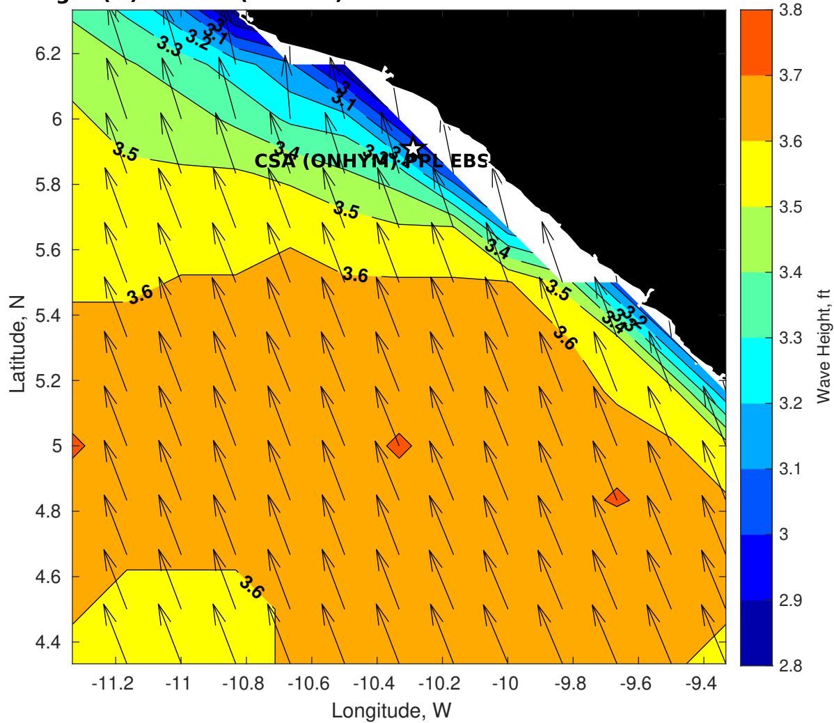
Wave Height (ft) for CSA (ONHYM) PPL EBS - Liberia at 03-Nov-2025 09:00:00
