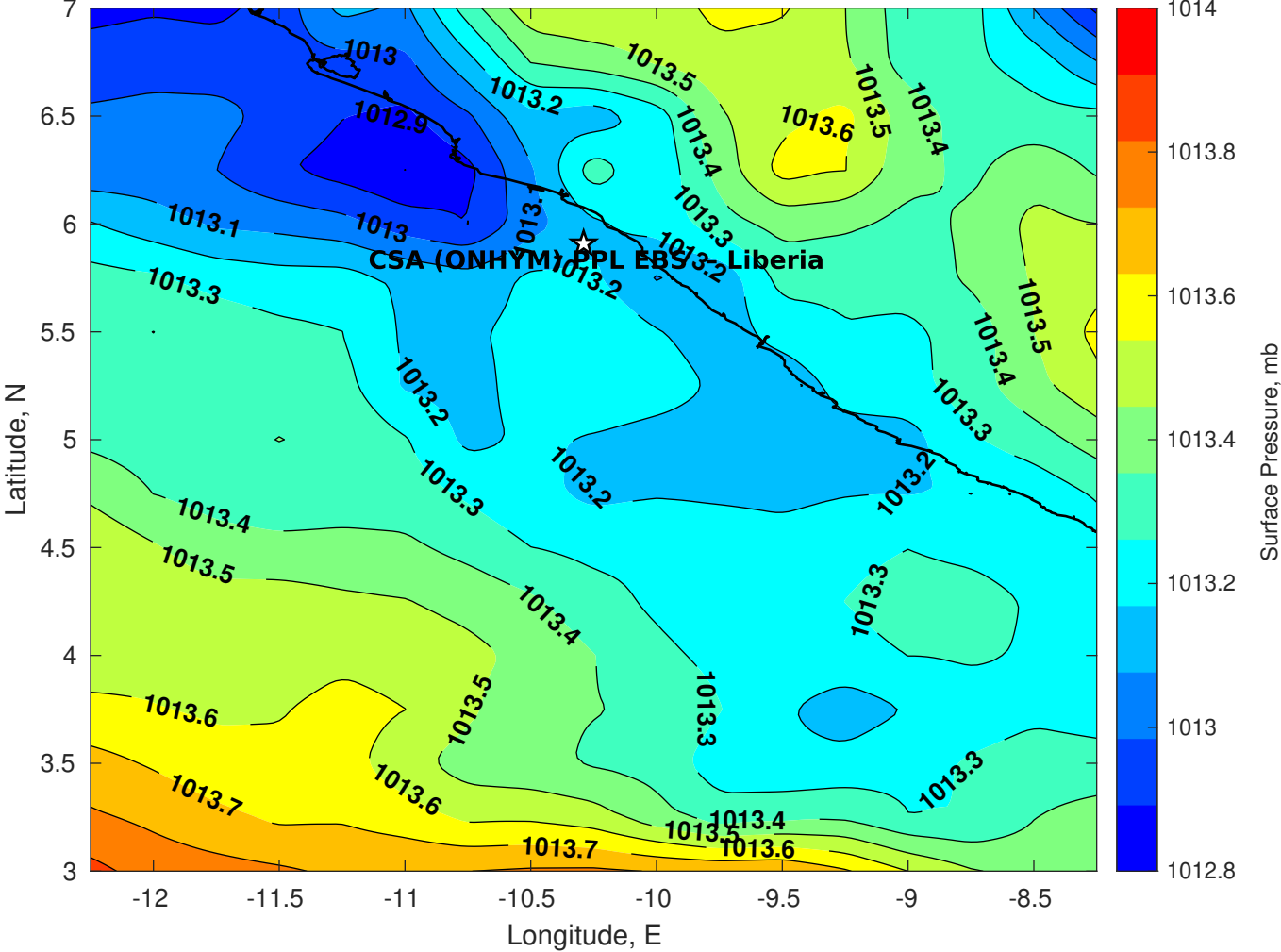
Surface Pressure (mb) for CSA (ONHYM) PPL EBS - Liberia at 03-Nov-2025 00:00:00
