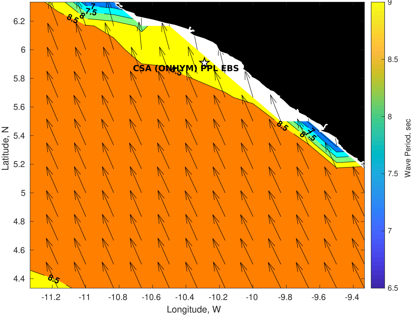
Wave Period (sec) for CSA (ONHYM) PPL EBS - Liberia at 03-Nov-2025 09:00:00
