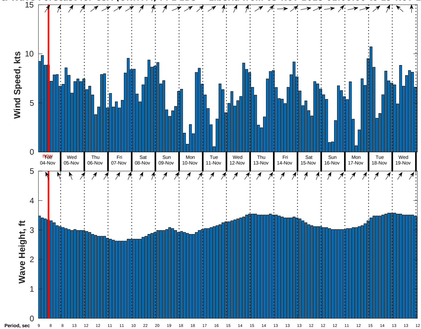
Wind & Wave Forecast for CSA (ONHYM) PPL EBS - Liberia from 03-Nov-2025 01:00:00 to 19-Nov-2025 01:00:00
