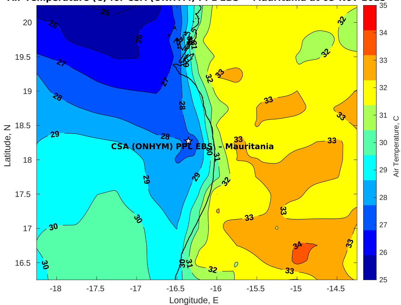
Air Temperature (C) for CSA (ONHYM) PPL EBS - Mauritania at 03-Nov-2025
