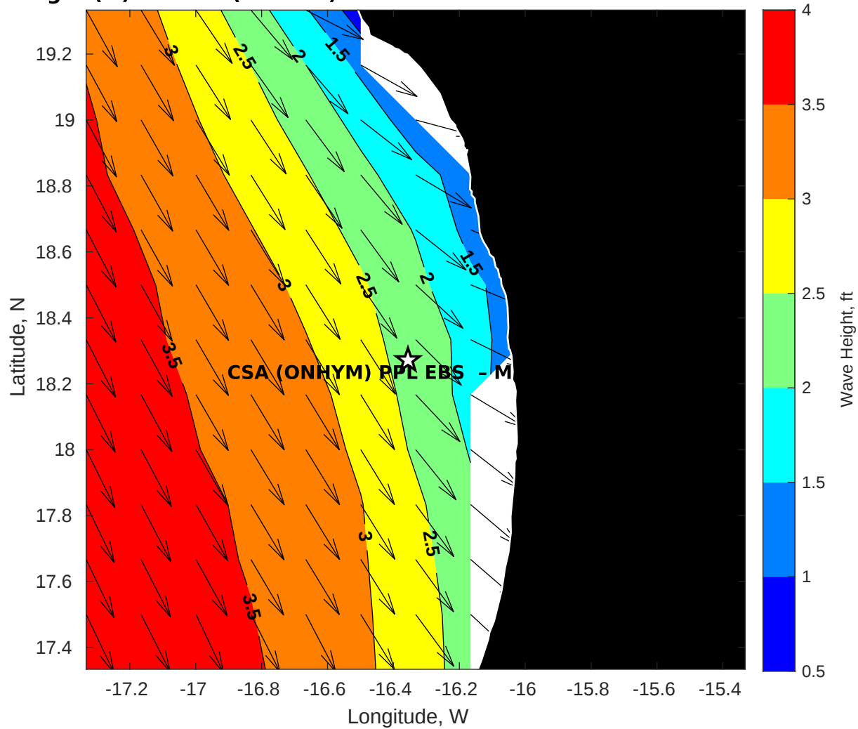
Wave Height (ft) for CSA (ONHYM) PPL EBS - Mauritania at 03-Nov-2025 09:00:00
