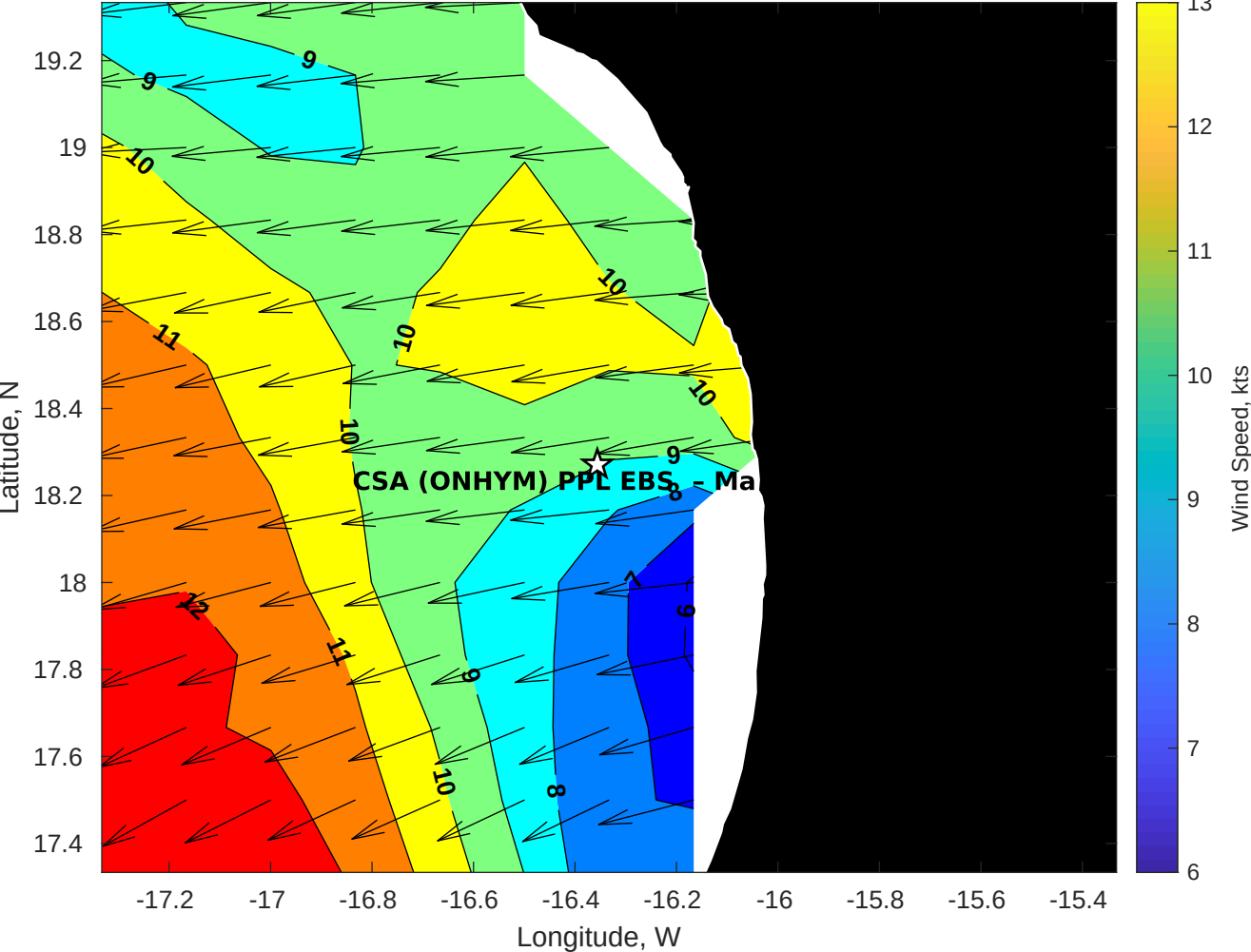
Winds (kts) for CSA (ONHYM) PPL EBS - Mauritania at 03-Nov-2025 09:00:00
