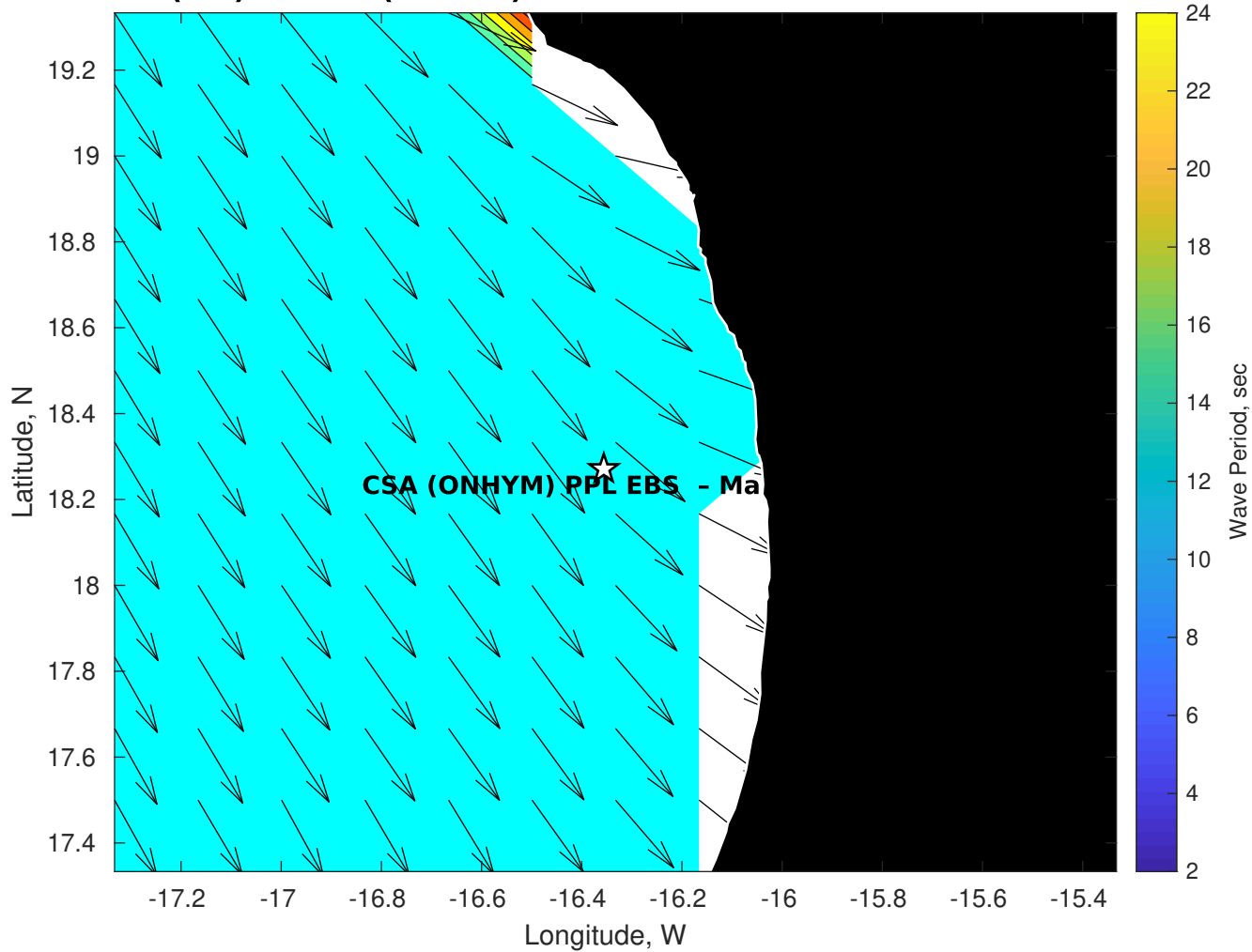
Wave Period (sec) for CSA (ONHYM) PPL EBS - Mauritania at 03-Nov-2025 09:00:00
