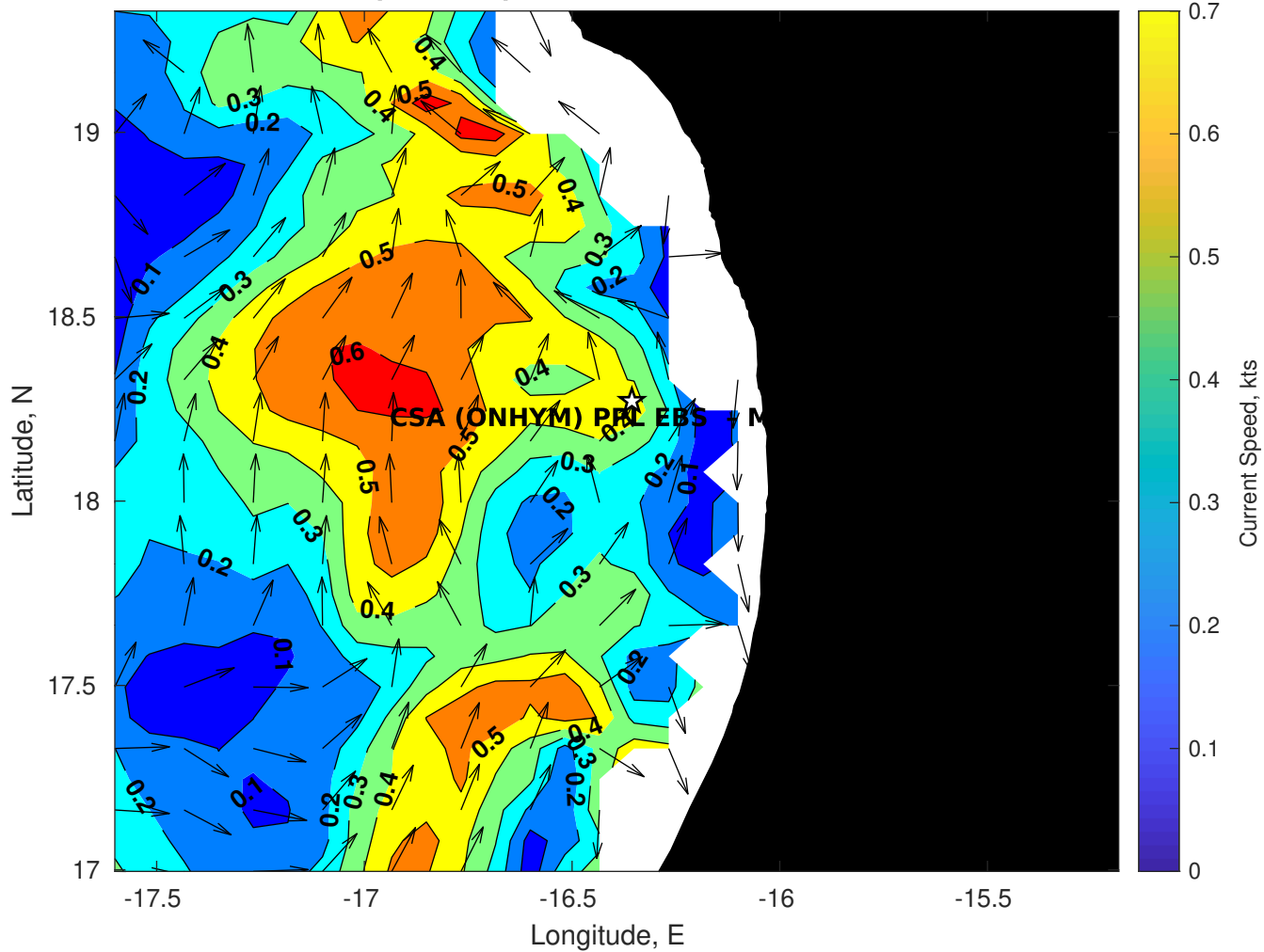
Surface Currents for CSA (ONHYM) PPL EBS - Mauritania at 02-Nov-2025 00:00:00
