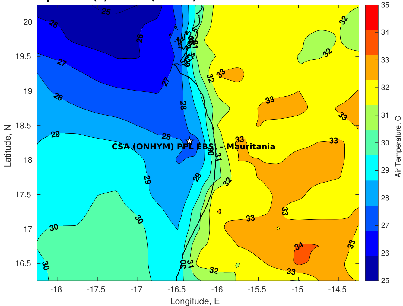
Air Temperature (C) for CSA (ONHYM) PPL EBS - Mauritania at 03-Nov-2025
