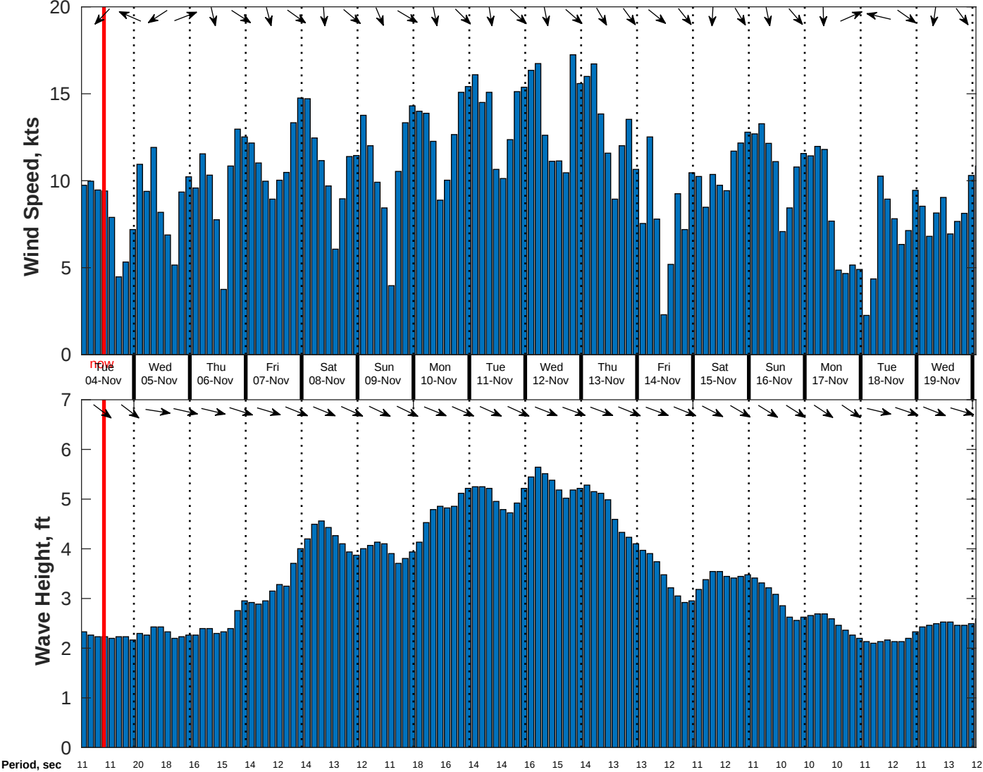
Wind & Wave Forecast for CSA (ONHYM) PPL EBS - Mauritania from 03-Nov-2025 01:00:00 to 19-Nov-2025 01:00:00
