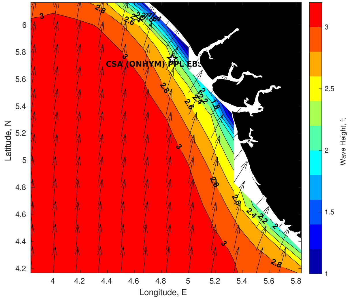
Wave Height (ft) for CSA (ONHYM) PPL EBS - Nigeria at 03-Nov-2025 09:00:00
