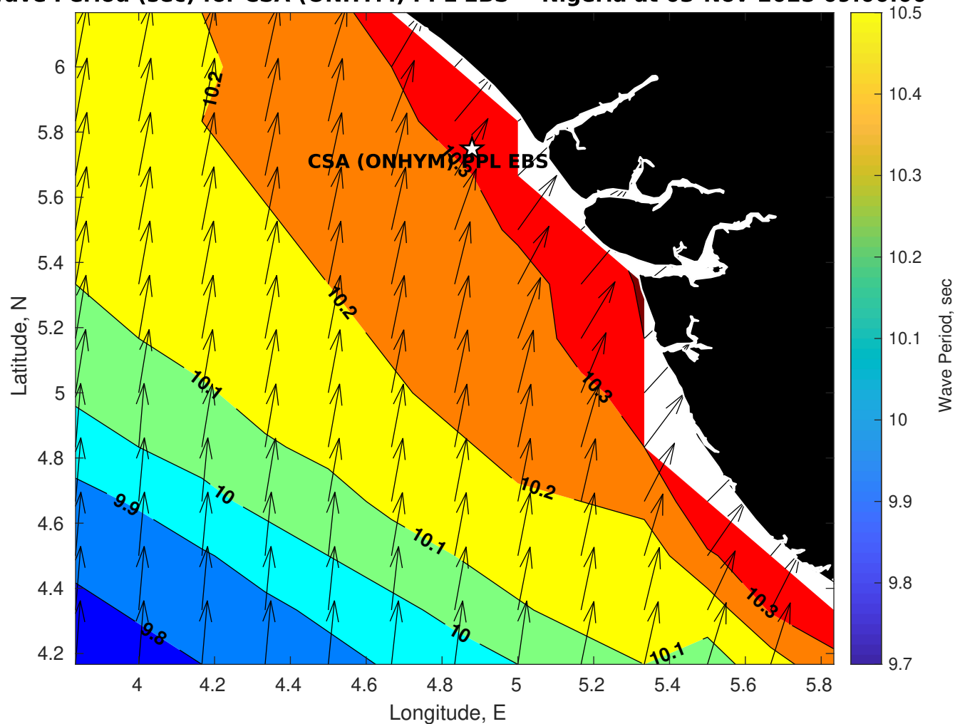
Wave Period (sec) for CSA (ONHYM) PPL EBS - Nigeria at 03-Nov-2025 09:00:00
