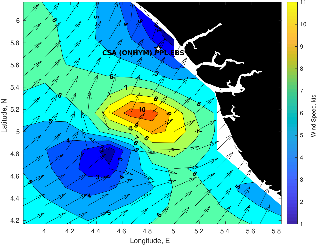
Winds (kts) for CSA (ONHYM) PPL EBS - Nigeria at 03-Nov-2025 09:00:00
