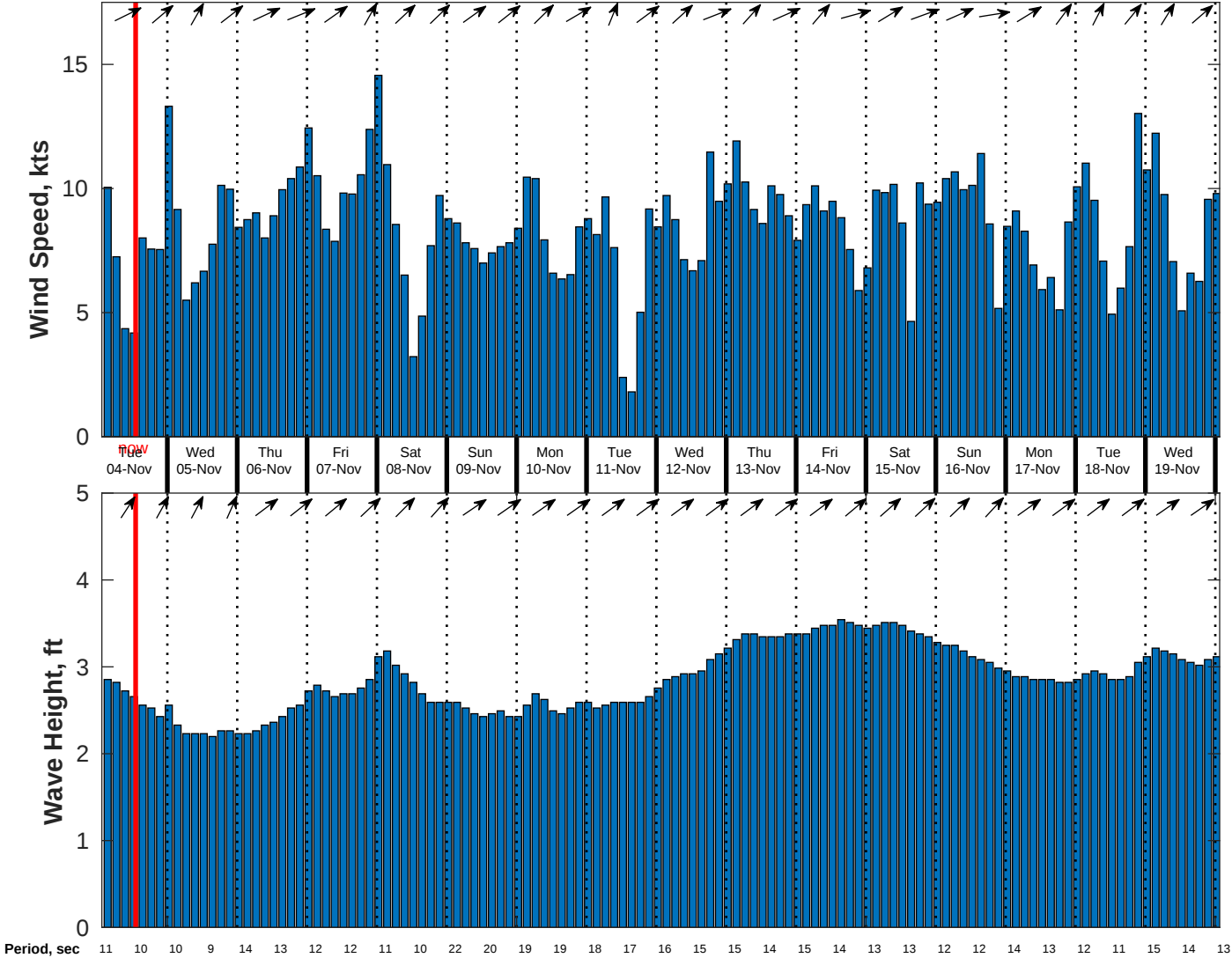
Wind & Wave Forecast for CSA (ONHYM) PPL EBS - Nigeria from 03-Nov-2025 02:00:00 to 19-Nov-2025 02:00:00
