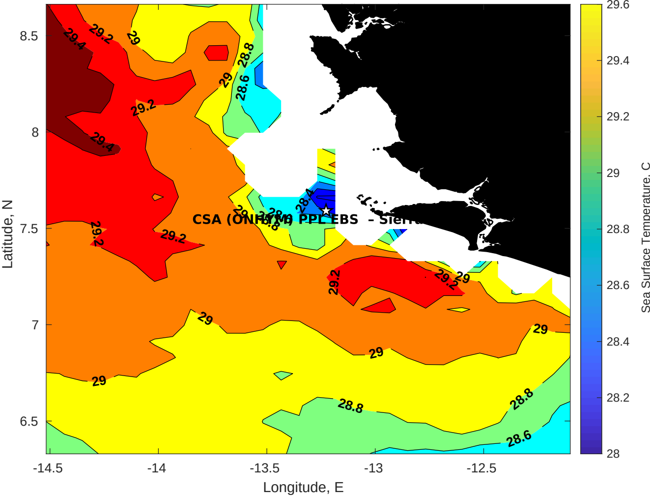
SST for CSA (ONHYM) PPL EBS - Sierra Leone at 02-Nov-2025 00:00:00
