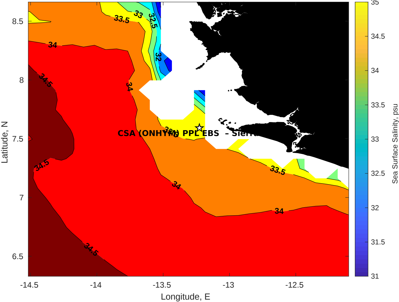
Surface Salinity for CSA (ONHYM) PPL EBS - Sierra Leone at 02-Nov-2025 00:00:00
