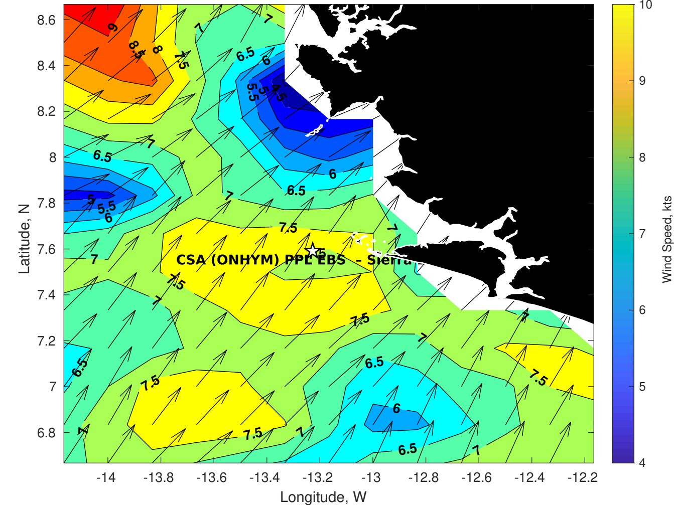
Winds (kts) for CSA (ONHYM) PPL EBS - Sierra Leone at 03-Nov-2025 09:00:00
