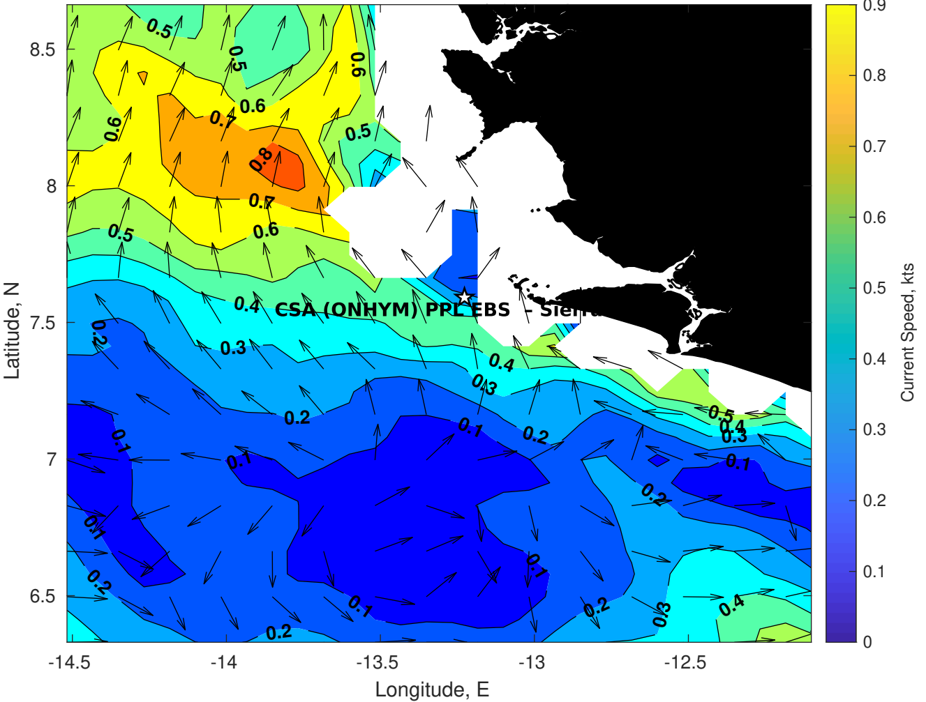
Surface Currents for CSA (ONHYM) PPL EBS - Sierra Leone at 02-Nov-2025 00:00:00
