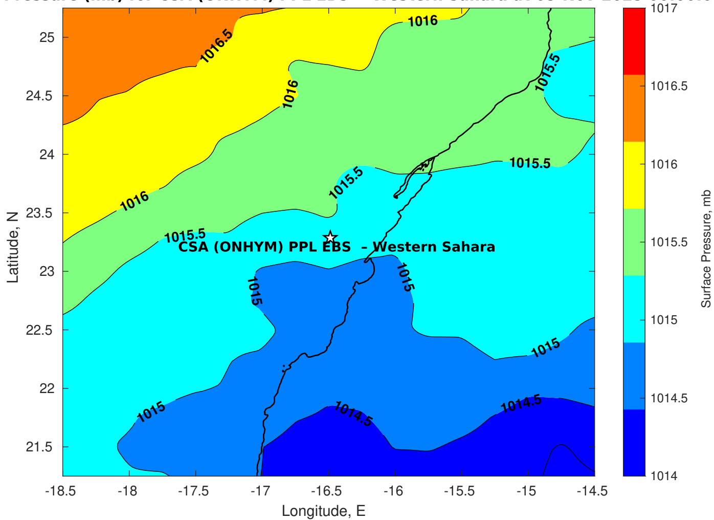
Surface Pressure (mb) for CSA (ONHYM) PPL EBS - Western Sahara at 05-Nov-2025 00:00:00
