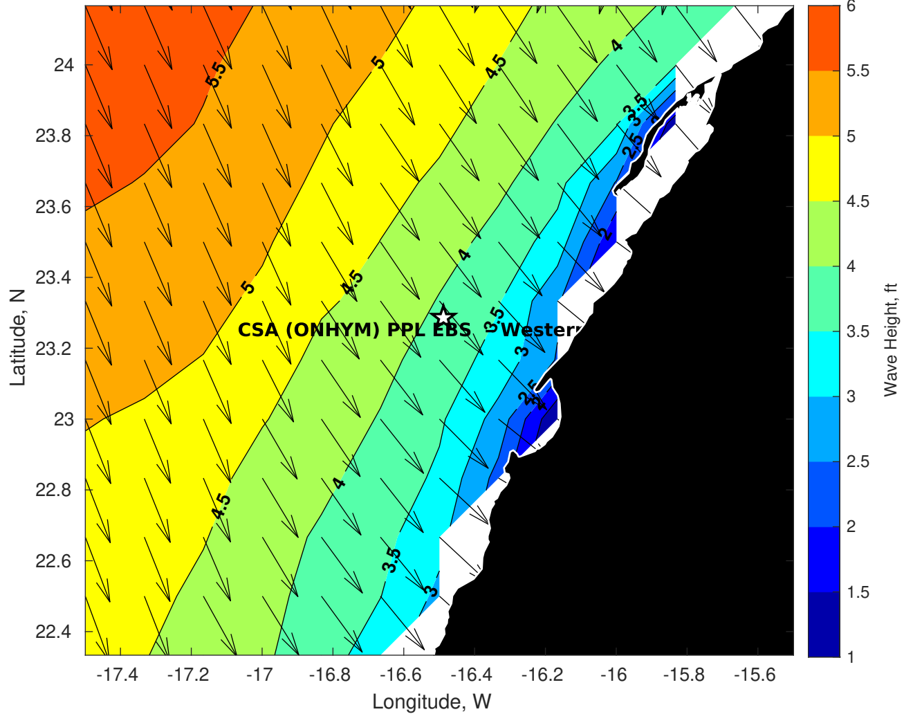
Wave Height (ft) for CSA (ONHYM) PPL EBS - Western Sahara at 03-Nov-2025 09:00:00
