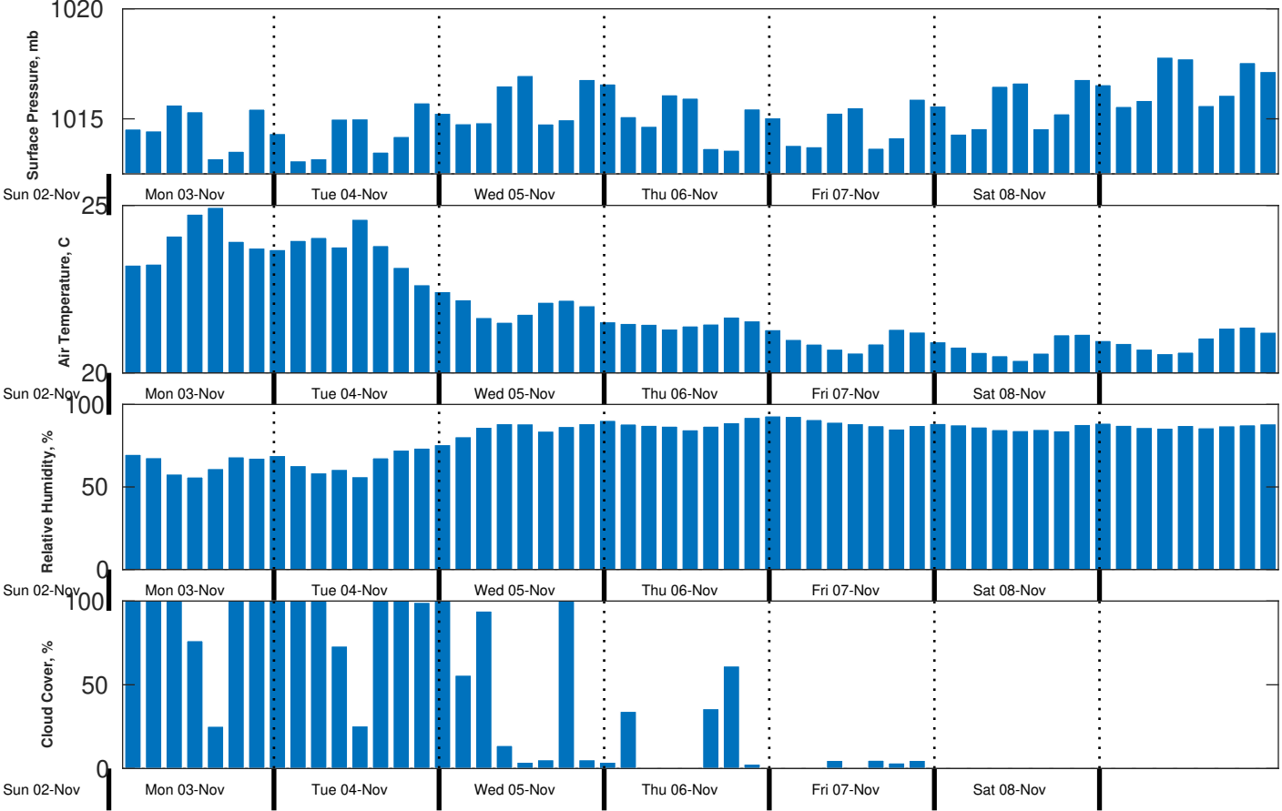
Met Forecast for CSA (ONHYM) PPL EBS - Western Sahara from 03-Nov-2025 00:00:00 to 10-Nov-2025 00:00:00
