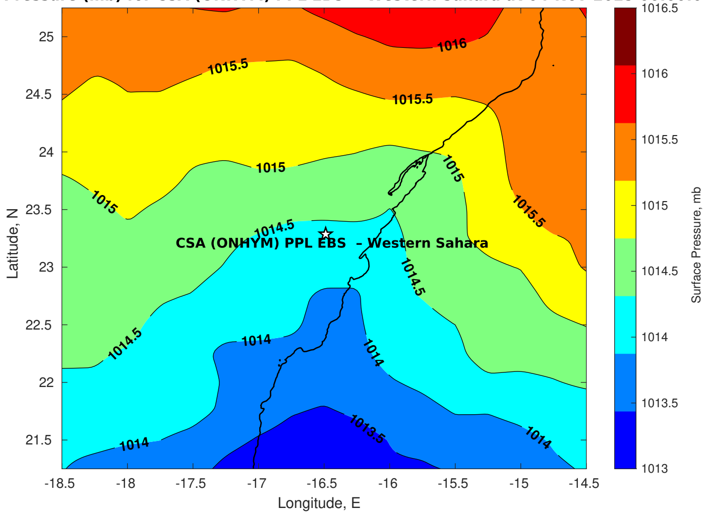
Surface Pressure (mb) for CSA (ONHYM) PPL EBS - Western Sahara at 04-Nov-2025 00:00:00
