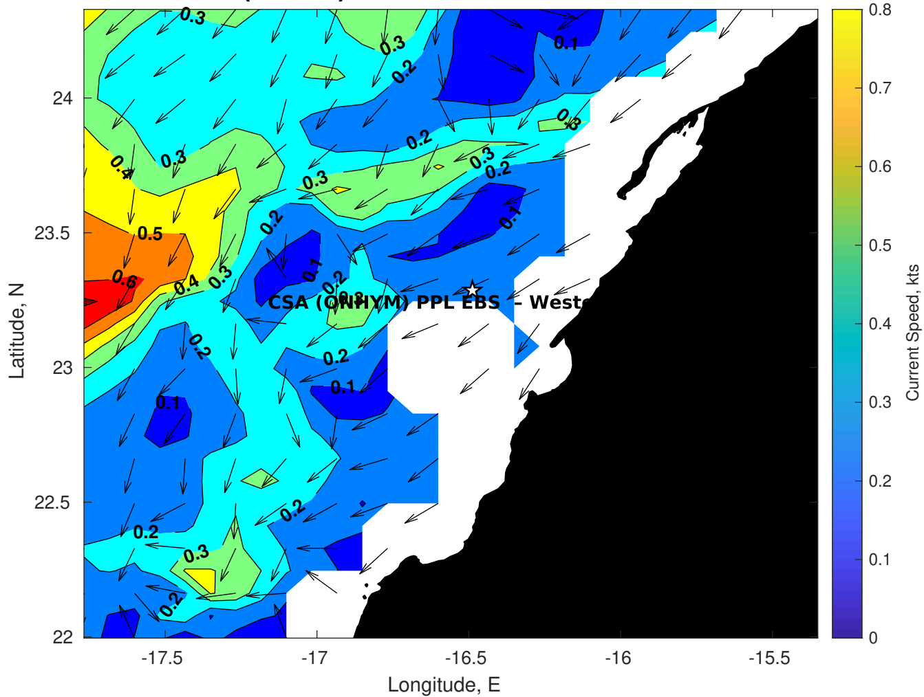
Surface Currents for CSA (ONHYM) PPL EBS - Western Sahara at 02-Nov-2025 00:00:00
