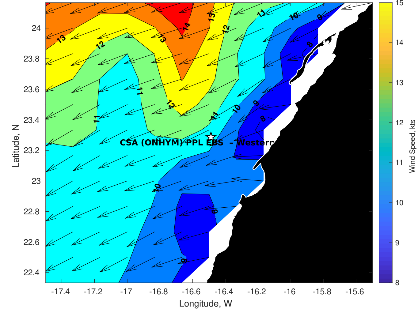
Winds (kts) for CSA (ONHYM) PPL EBS - Western Sahara at 03-Nov-2025 09:00:00
