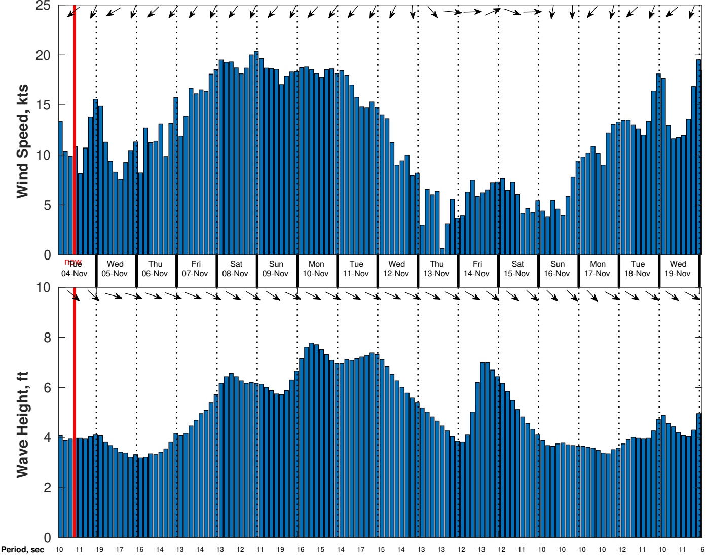
Wind & Wave Forecast for CSA (ONHYM) PPL EBS - Western Sahara from 03-Nov-2025 01:00:00 to 19-Nov-2025 01:00:00
