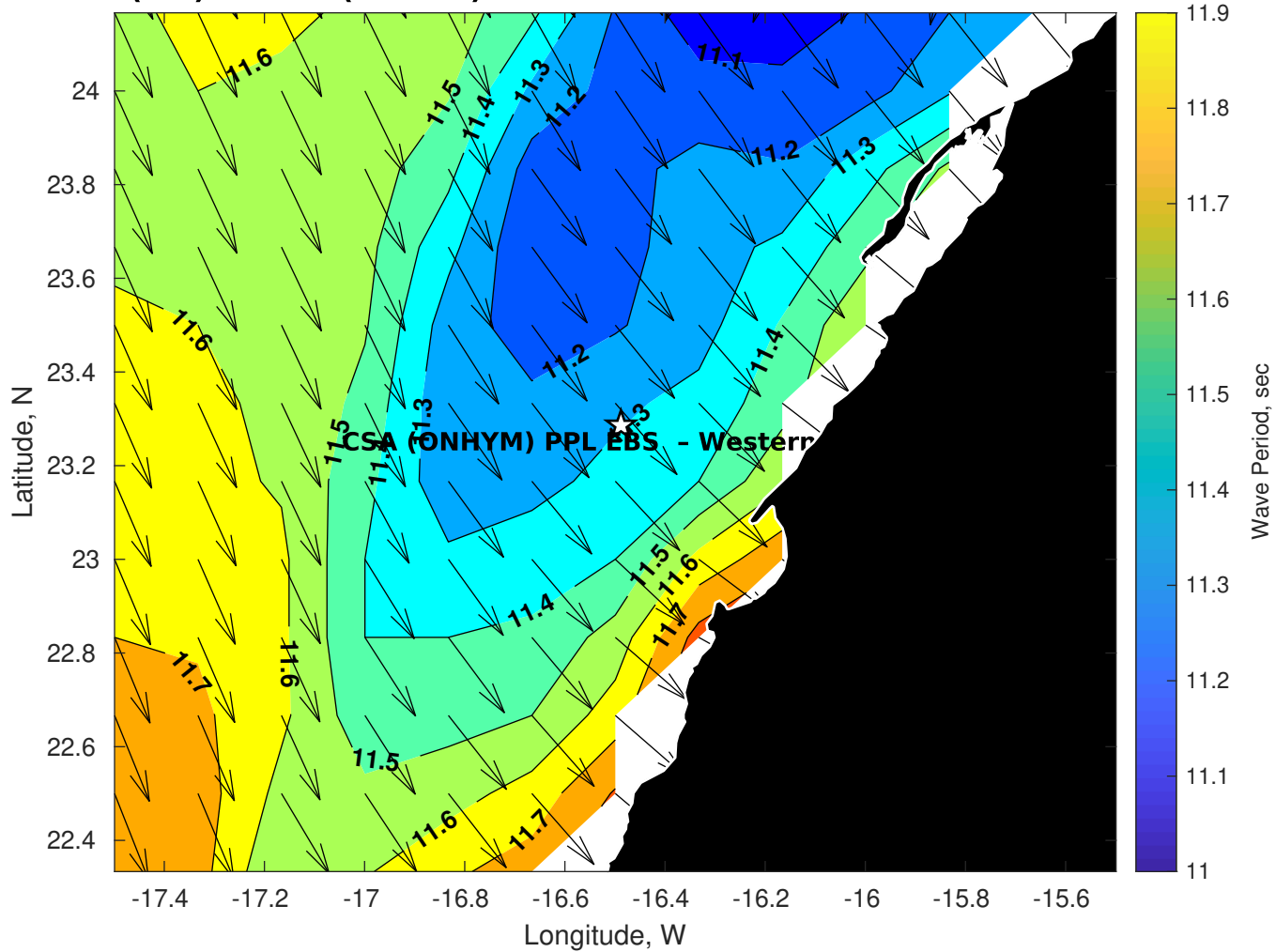
Wave Period (sec) for CSA (ONHYM) PPL EBS - Western Sahara at 03-Nov-2025 09:00:00
