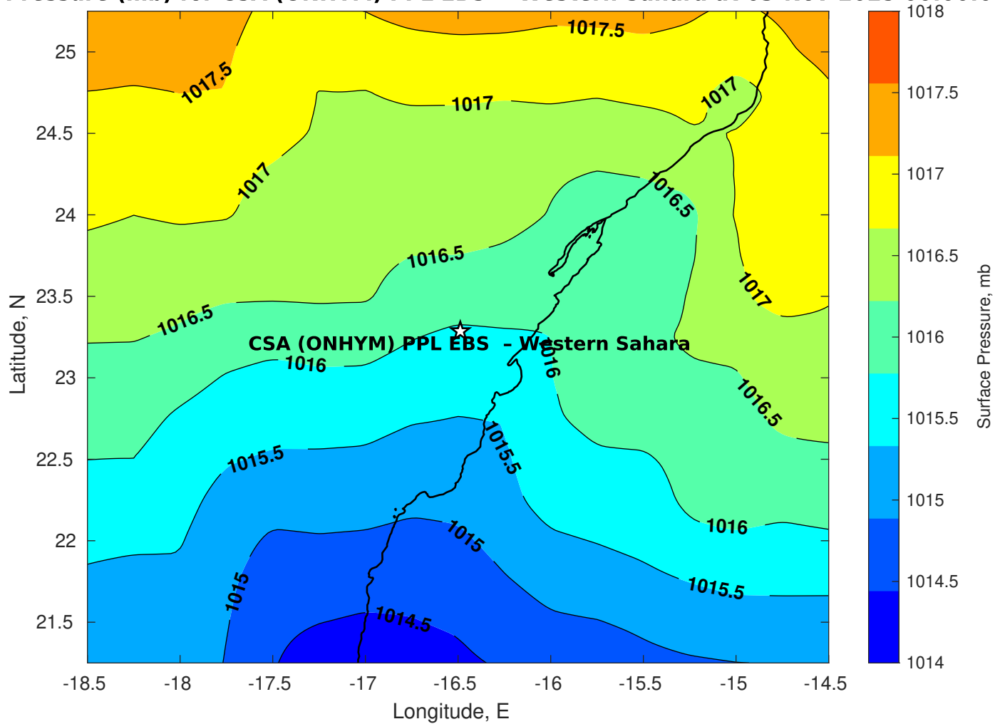
Surface Pressure (mb) for CSA (ONHYM) PPL EBS - Western Sahara at 03-Nov-2025 00:00:00
