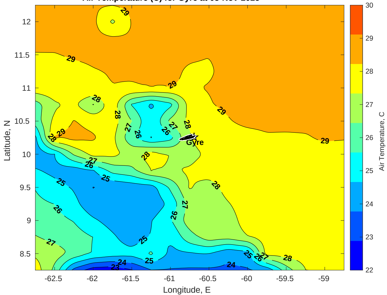
Air Temperature (C) for Gyre at 03-Nov-2025
