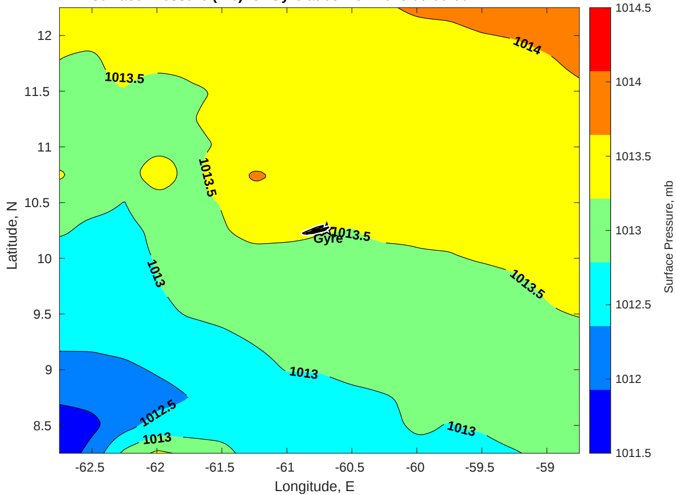
Surface Pressure (mb) for Gyre at 05-Nov-2025 00:00:00
