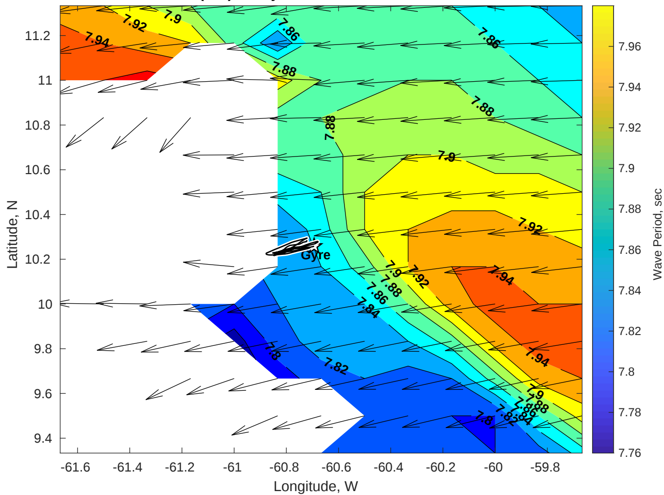
Wave Period (sec) for Gyre at 03-Nov-2025 09:00:00
