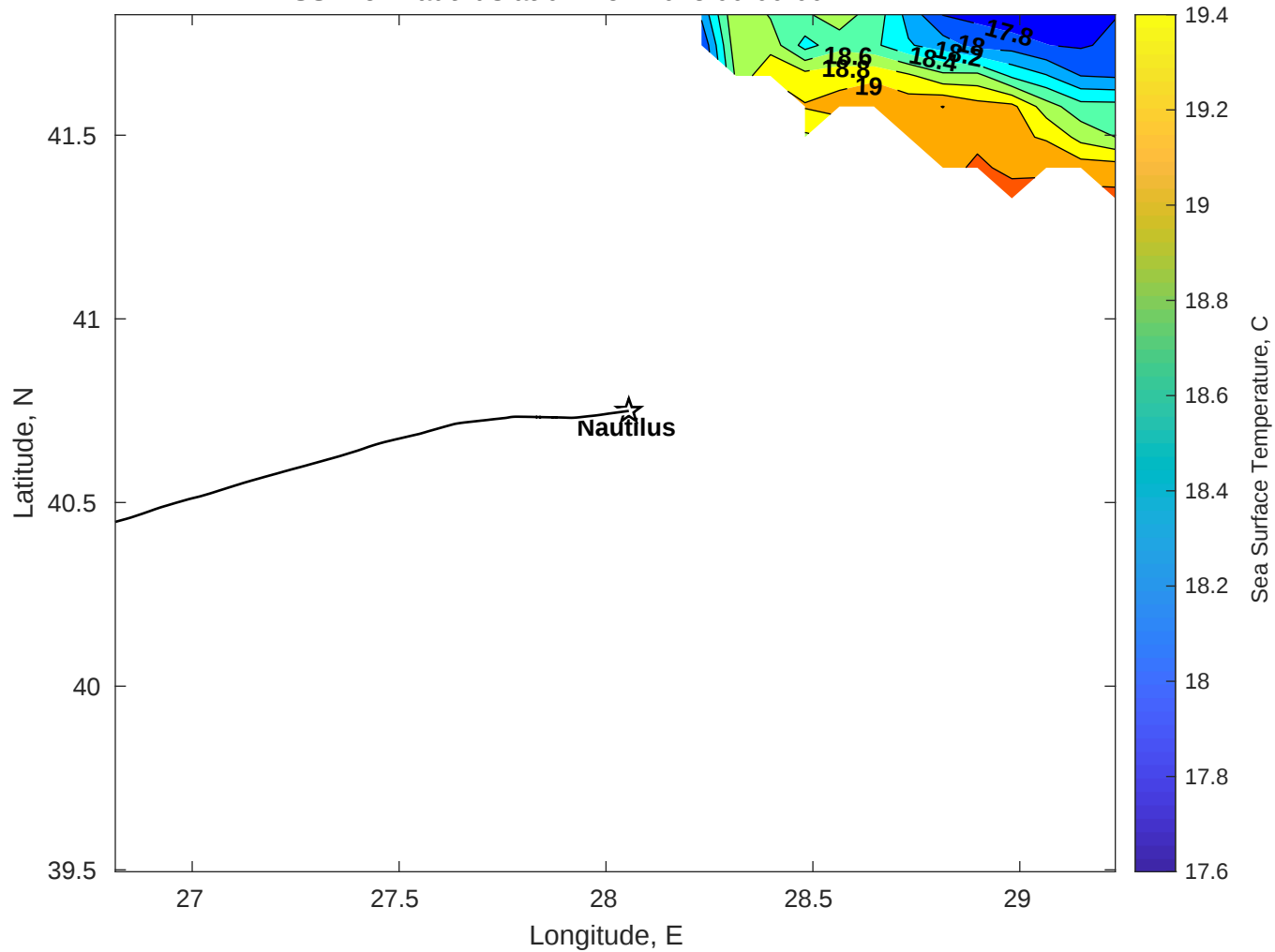
SST for Nautilus at 02-Nov-2025 00:00:00
