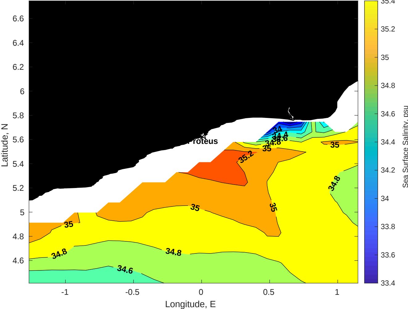
Surface Salinity for Proteus at 02-Nov-2025 00:00:00
