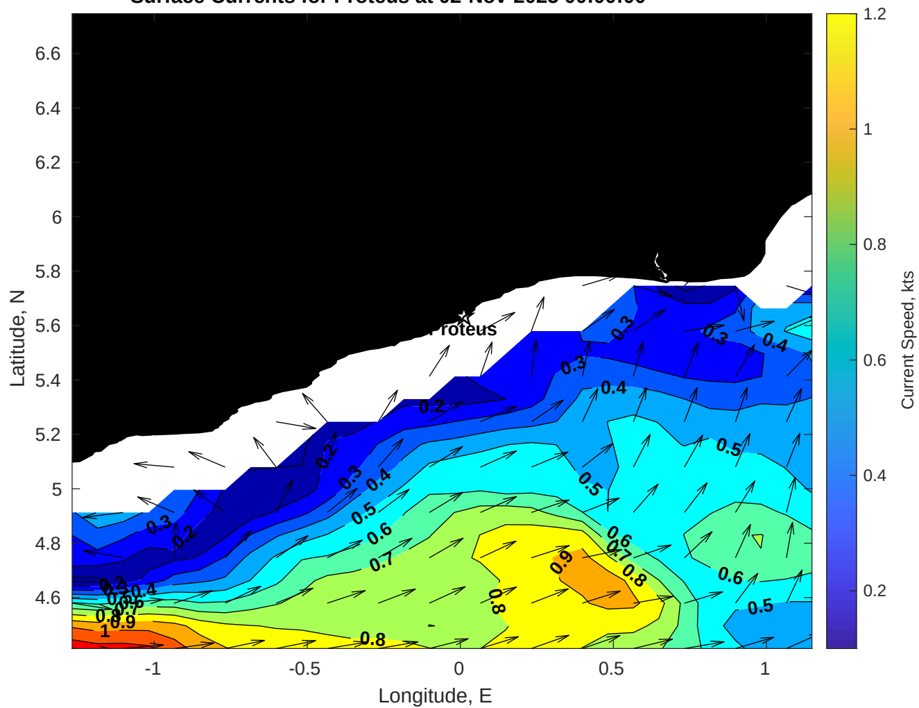
Surface Currents for Proteus at 02-Nov-2025 00:00:00
