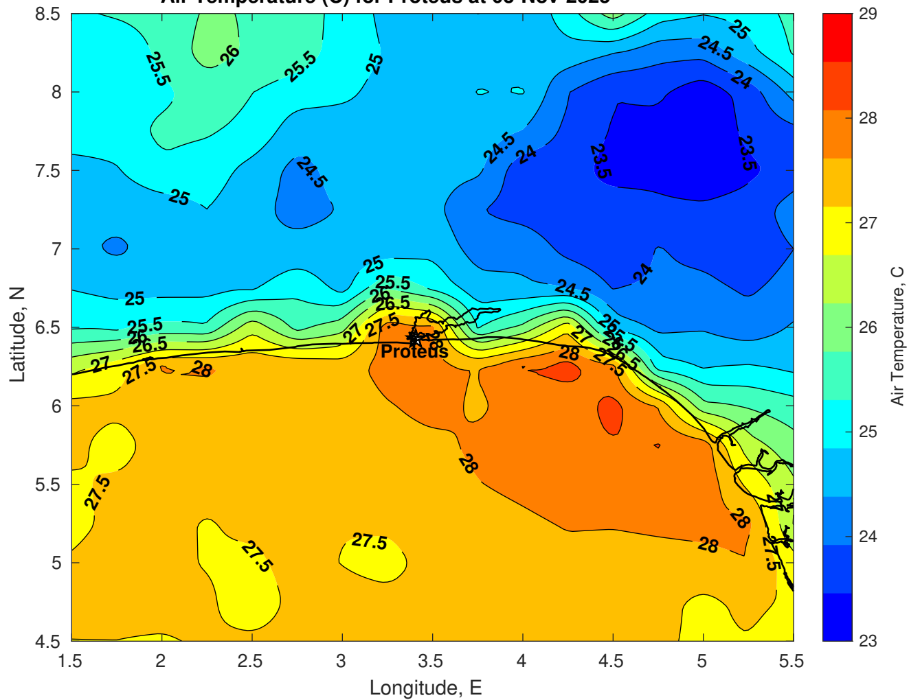
Air Temperature (C) for Proteus at 03-Nov-2025
