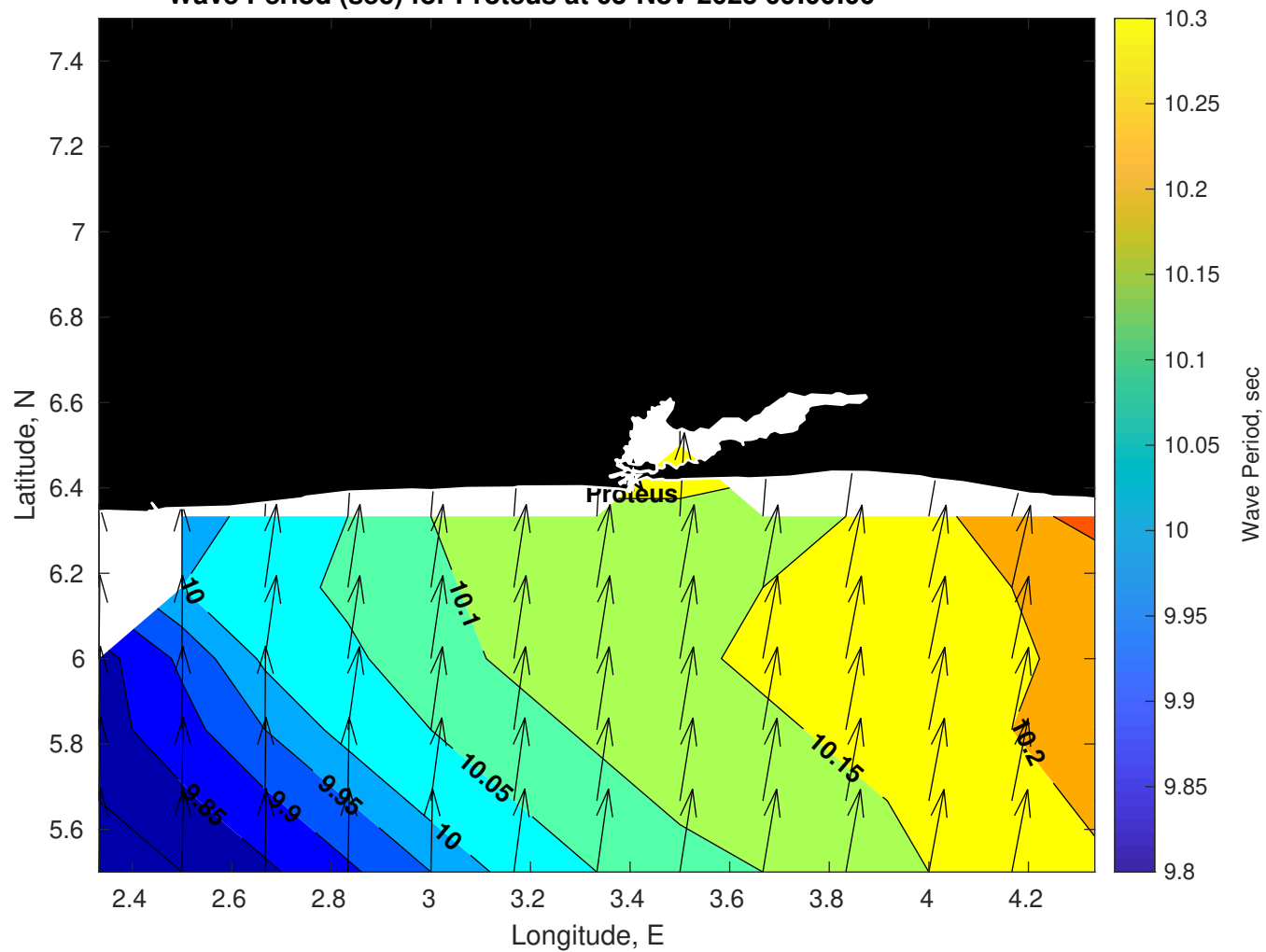
Wave Period (sec) for Proteus at 03-Nov-2025 09:00:00
