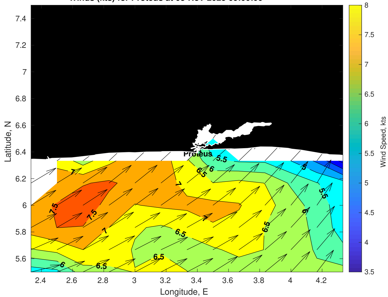
Winds (kts) for Proteus at 03-Nov-2025 09:00:00
