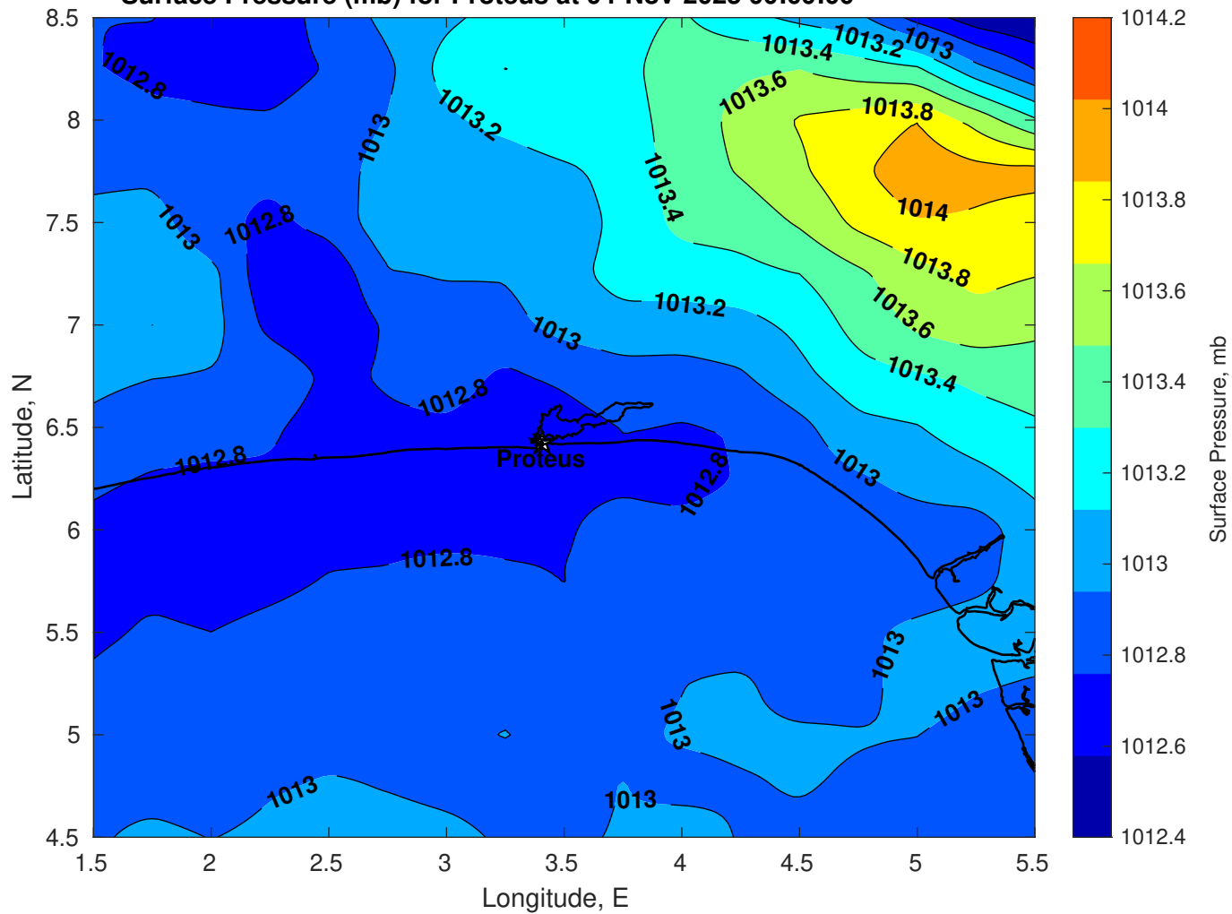
Surface Pressure (mb) for Proteus at 04-Nov-2025 00:00:00
