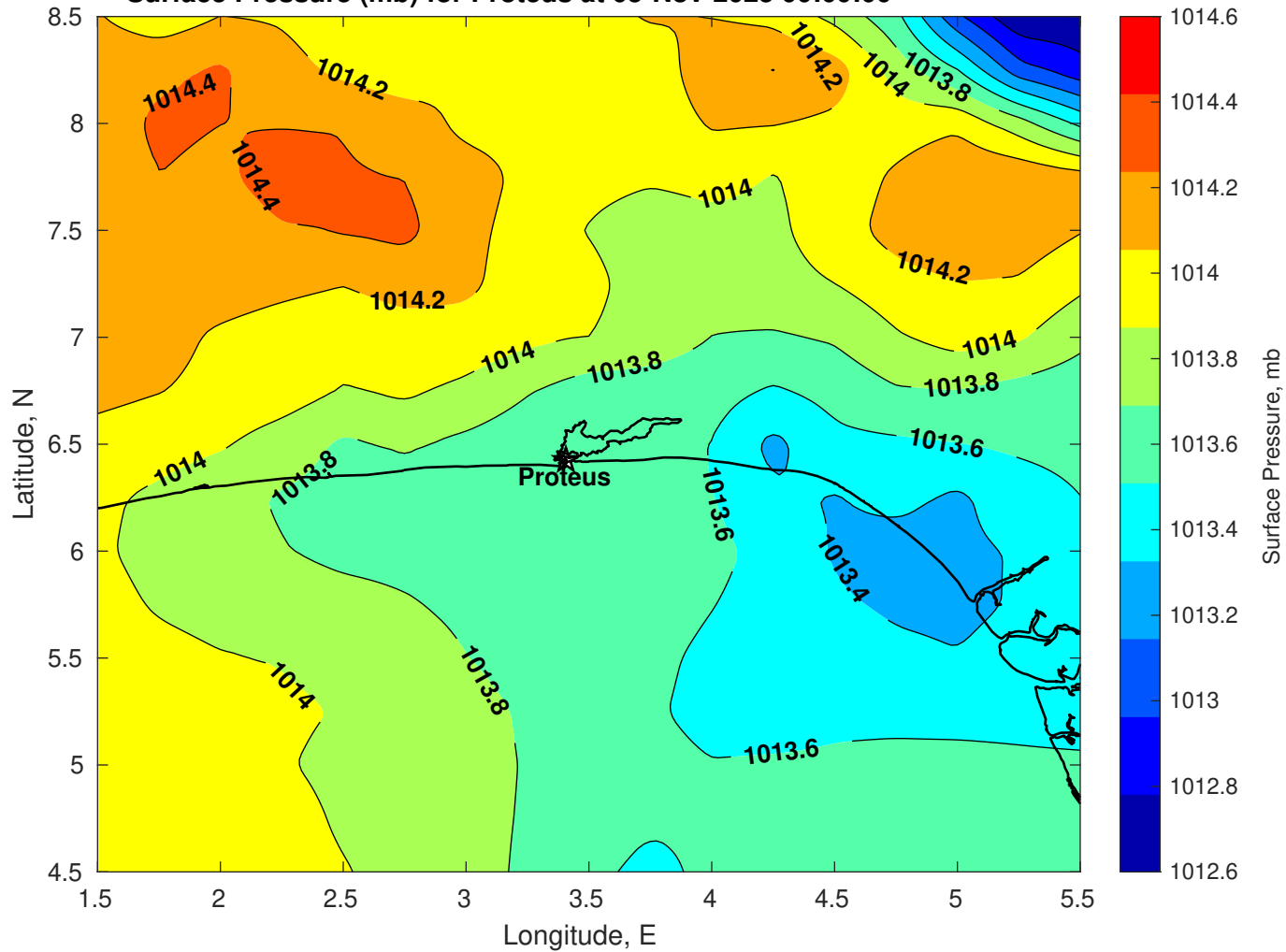
Surface Pressure (mb) for Proteus at 05-Nov-2025 00:00:00
