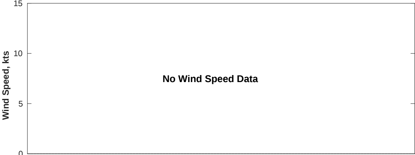
Wind & Wave Forecast for Proteus from 03-Nov-2025 01:00:00 to 19-Nov-2025 01:00:00
