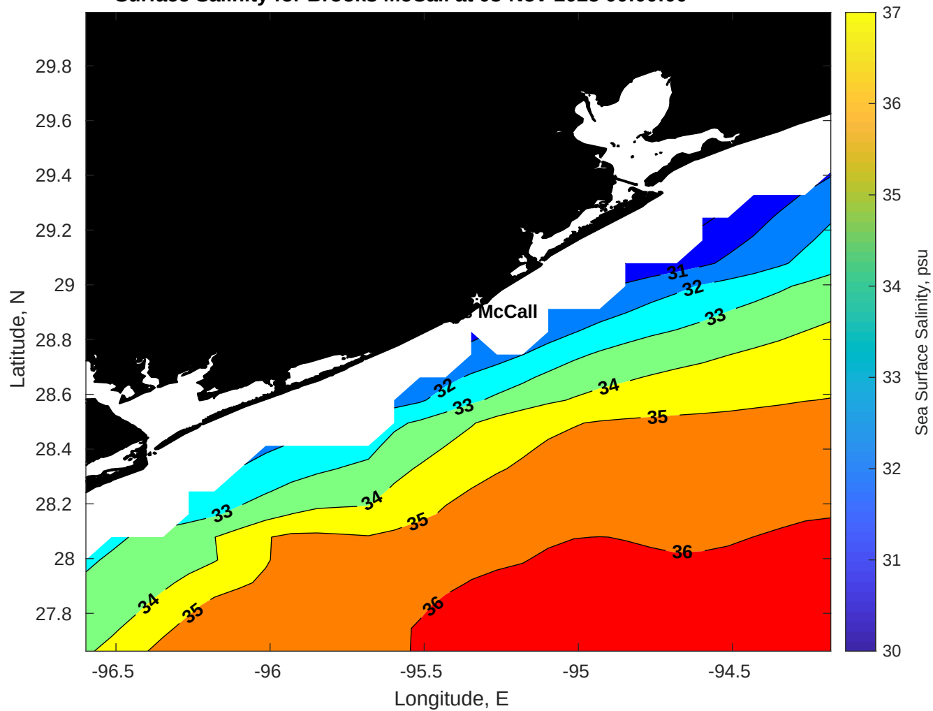
Surface Salinity for Brooks McCall at 03-Nov-2025 00:00:00
