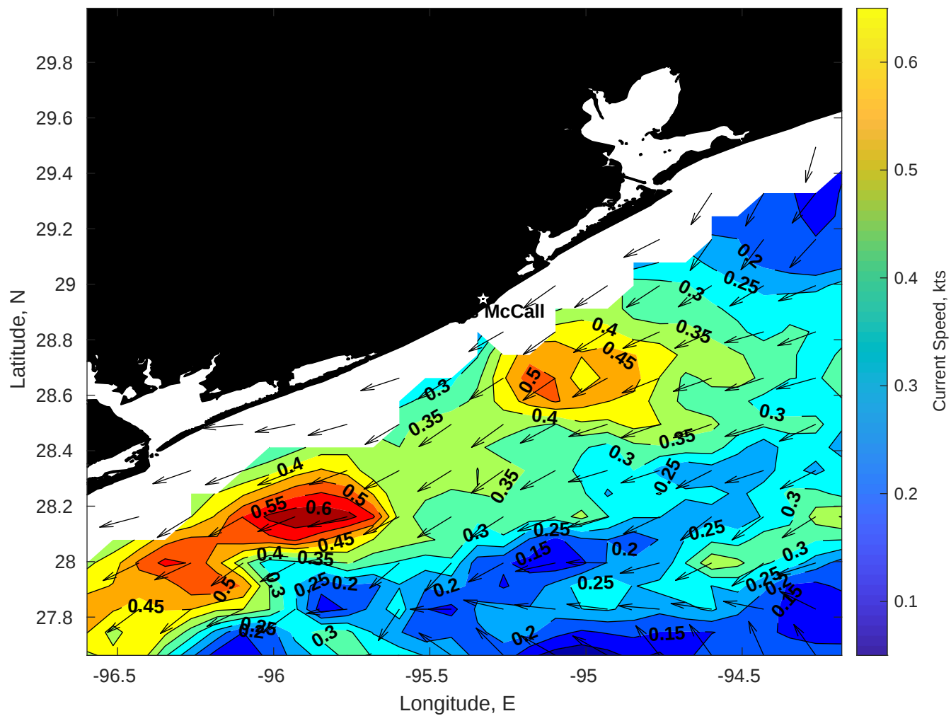
Surface Currents for Brooks McCall at 03-Nov-2025 00:00:00
