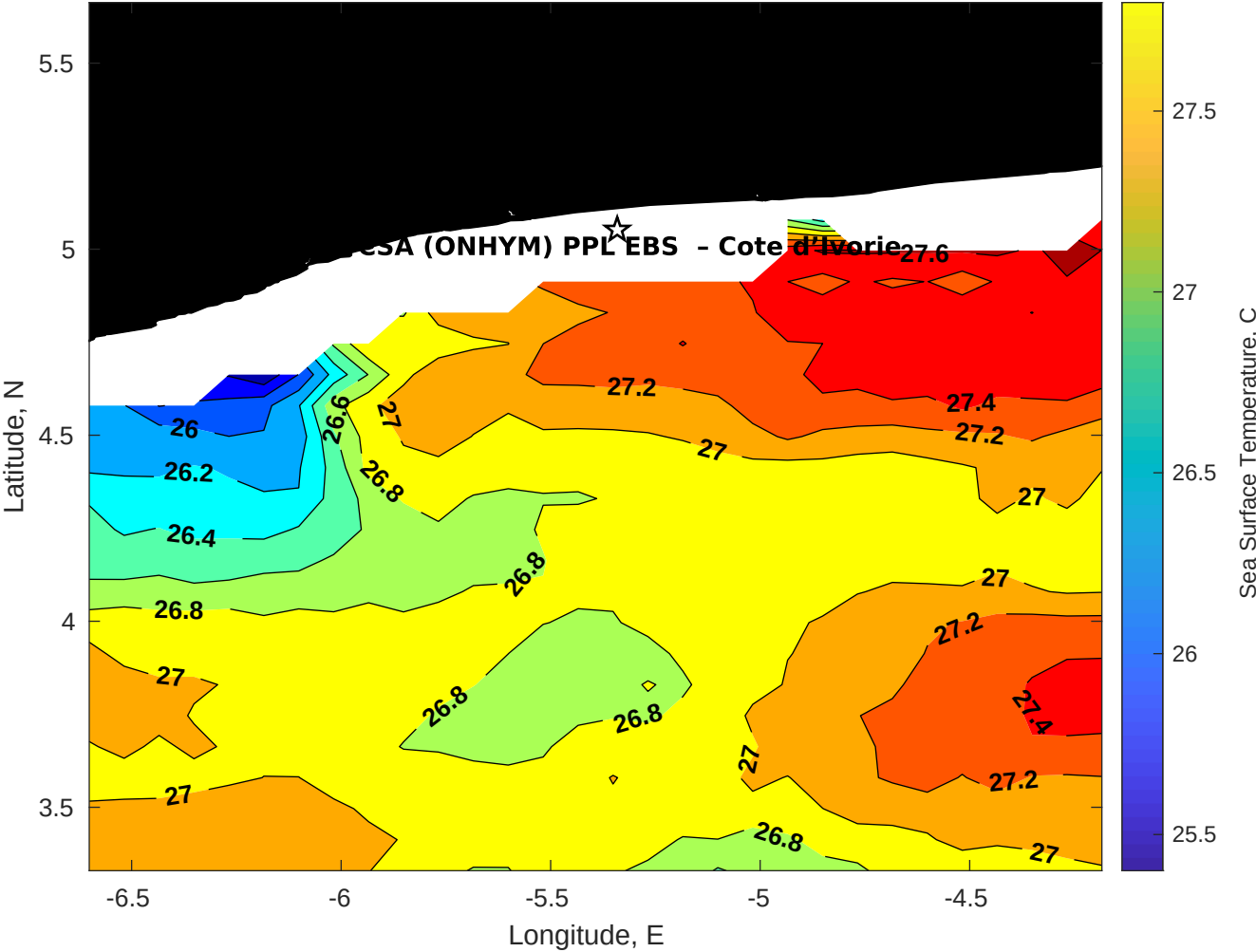
SST for CSA (ONHYM) PPL EBS - Cote d'Ivoire at 03-Nov-2025 00:00:00
