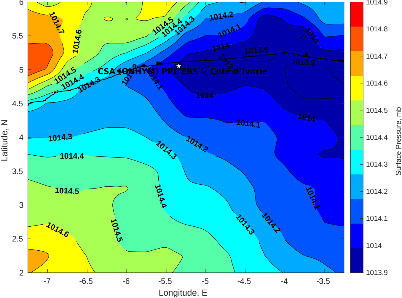
Surface Pressure (mb) for CSA (ONHYM) PPL EBS - Cote d'Ivoire at 05-Nov-2025 00:00:00
