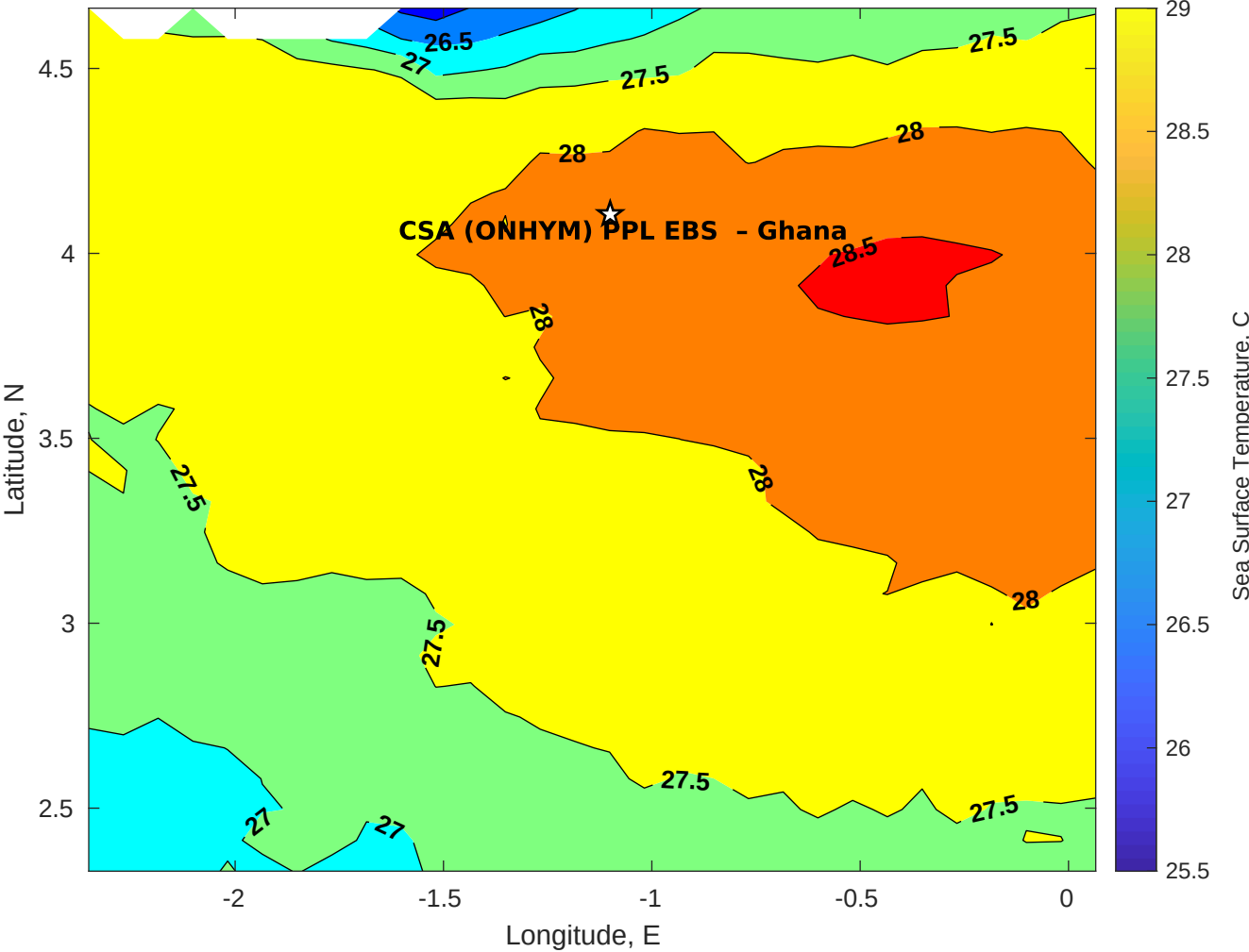
SST for CSA (ONHYM) PPL EBS - Ghana at 03-Nov-2025 00:00:00
