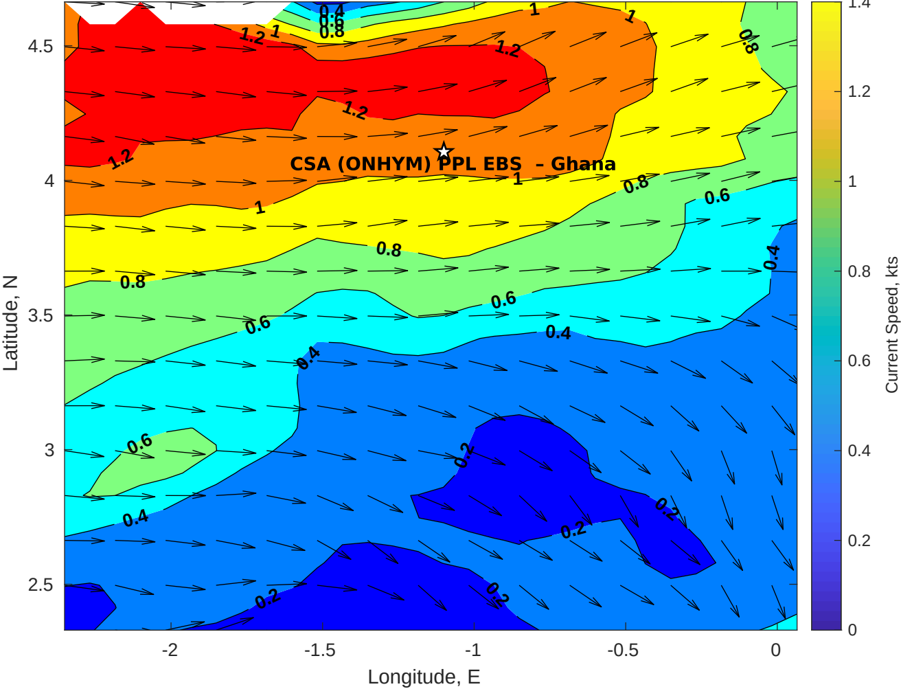
Surface Currents for CSA (ONHYM) PPL EBS - Ghana at 03-Nov-2025 00:00:00
