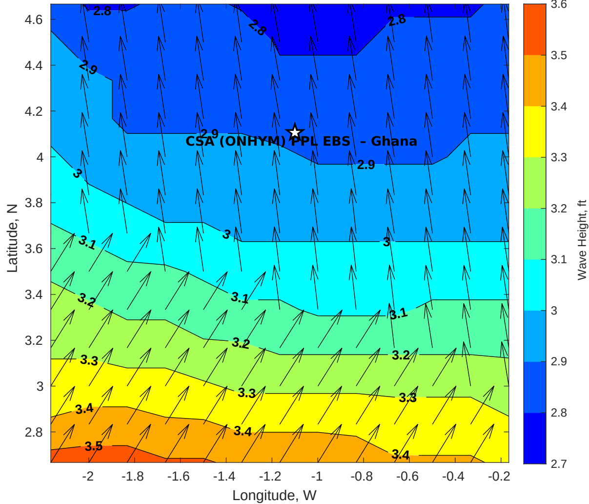
Wave Height (ft) for CSA (ONHYM) PPL EBS - Ghana at 04-Nov-2025 09:00:00
