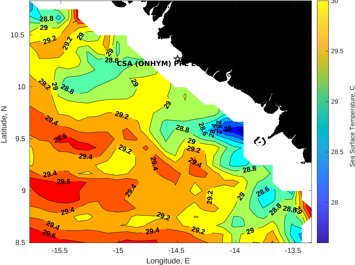
SST for CSA (ONHYM) PPL EBS - Guinea at 03-Nov-2025 00:00:00
