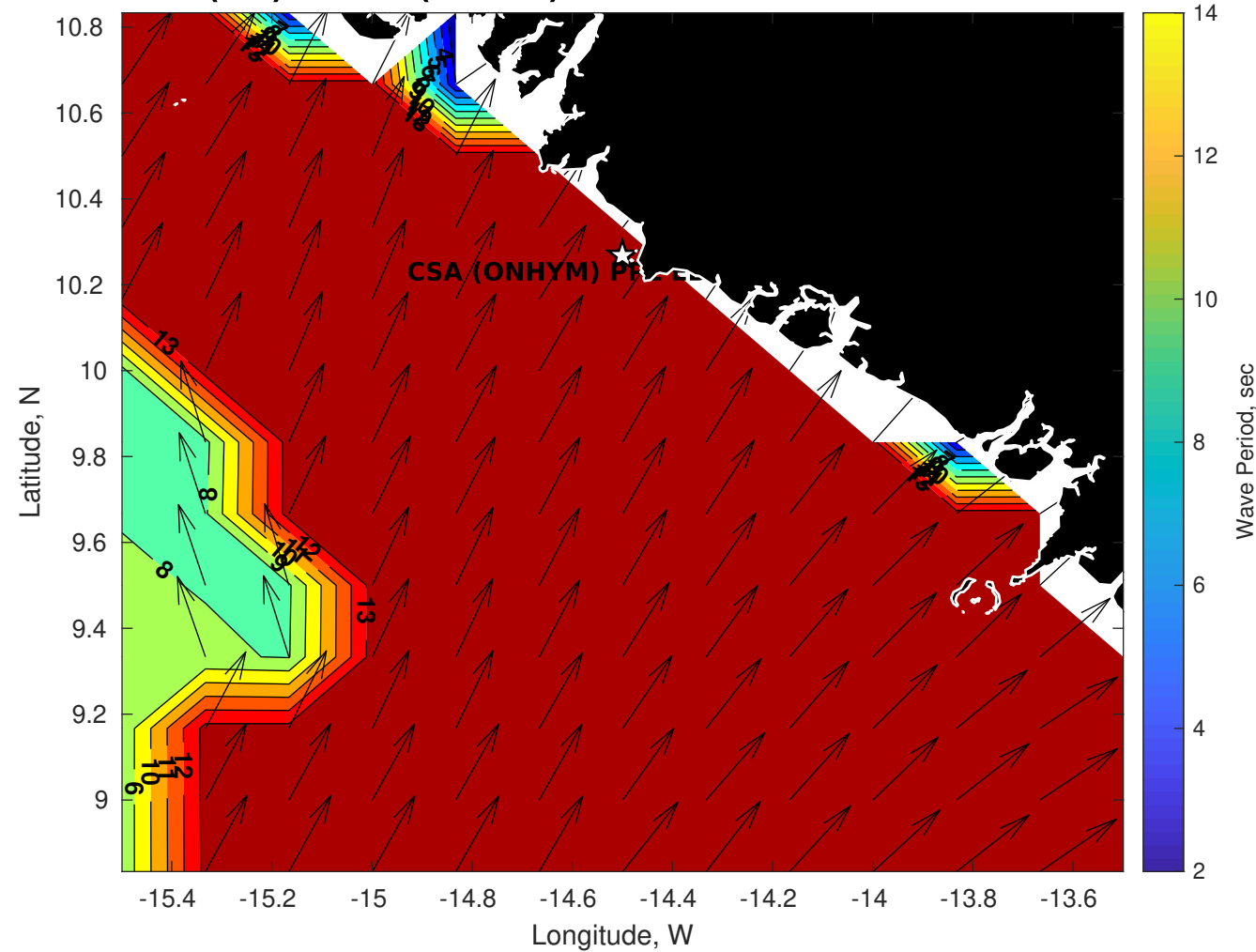
Wave Period (sec) for CSA (ONHYM) PPL EBS - Guinea at 04-Nov-2025 09:00:00
