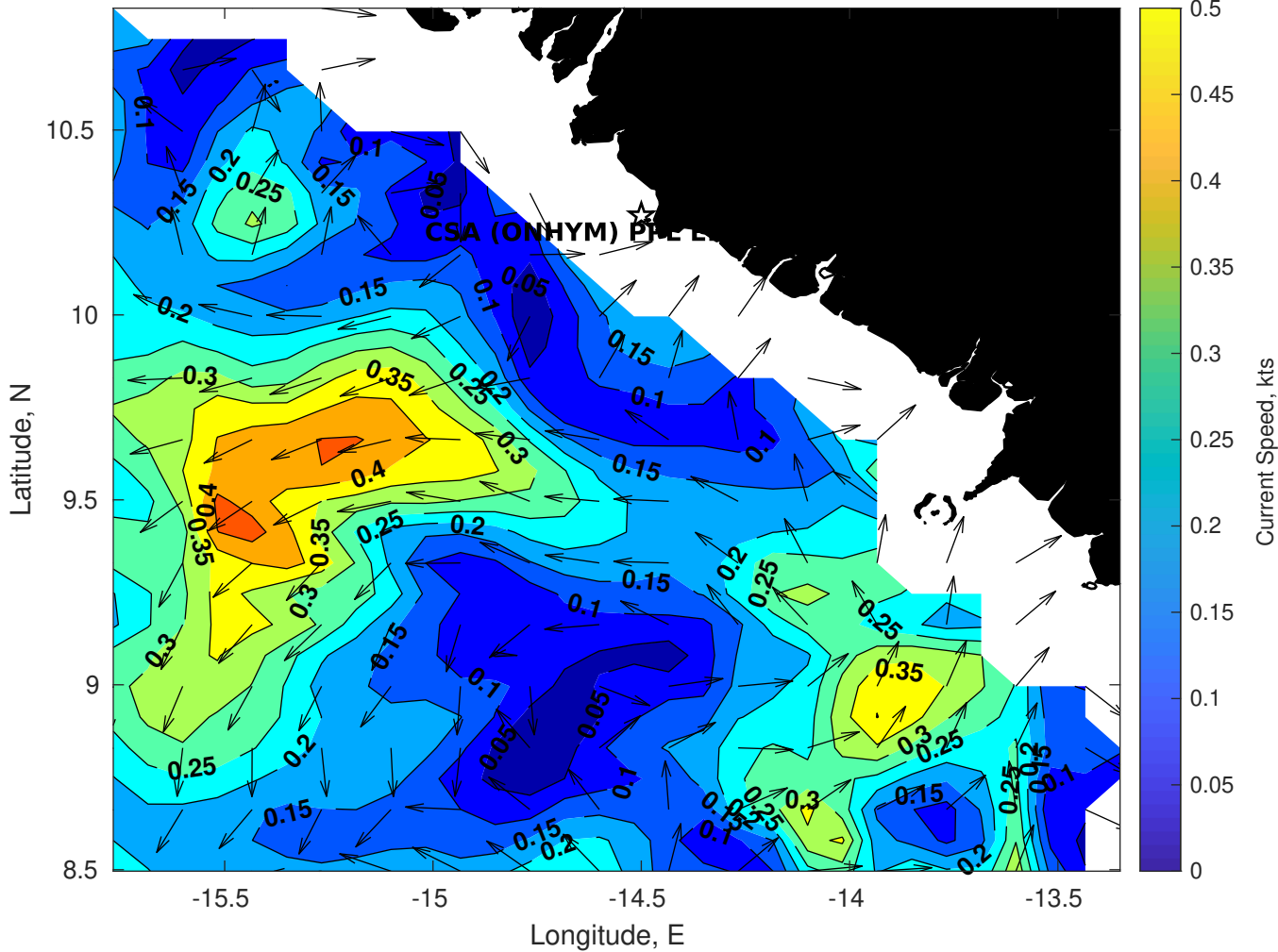
Surface Currents for CSA (ONHYM) PPL EBS - Guinea at 03-Nov-2025 00:00:00
