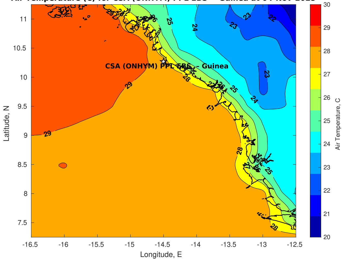
Air Temperature (C) for CSA (ONHYM) PPL EBS - Guinea at 04-Nov-2025
