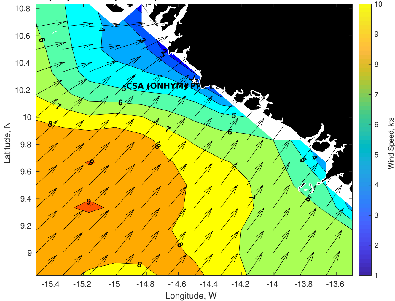
Winds (kts) for CSA (ONHYM) PPL EBS - Guinea at 04-Nov-2025 09:00:00
