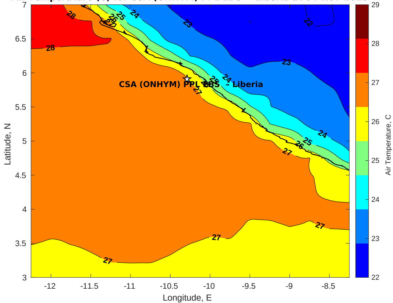
Air Temperature (C) for CSA (ONHYM) PPL EBS - Liberia at 04-Nov-2025
