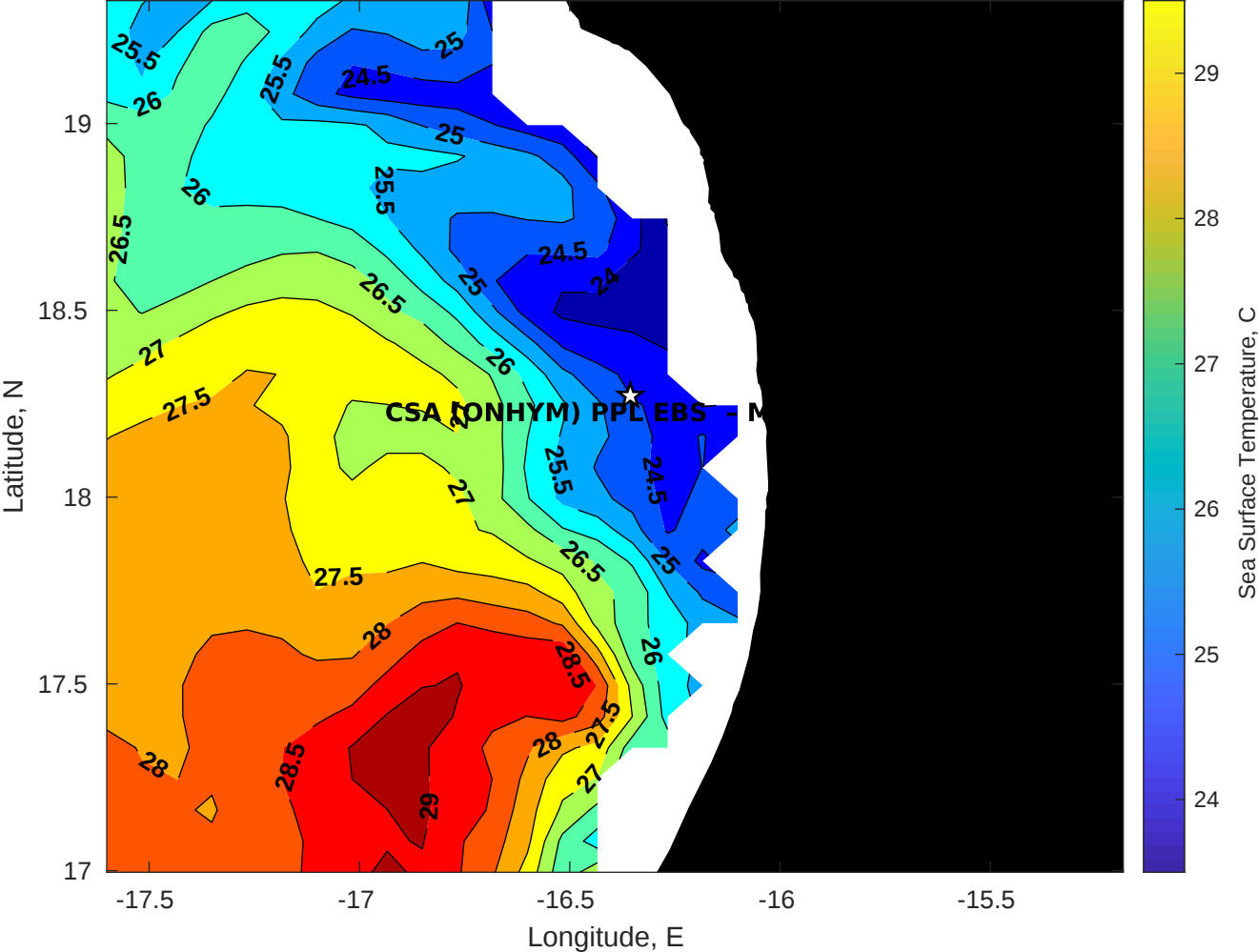
SST for CSA (ONHYM) PPL EBS - Mauritania at 03-Nov-2025 00:00:00
