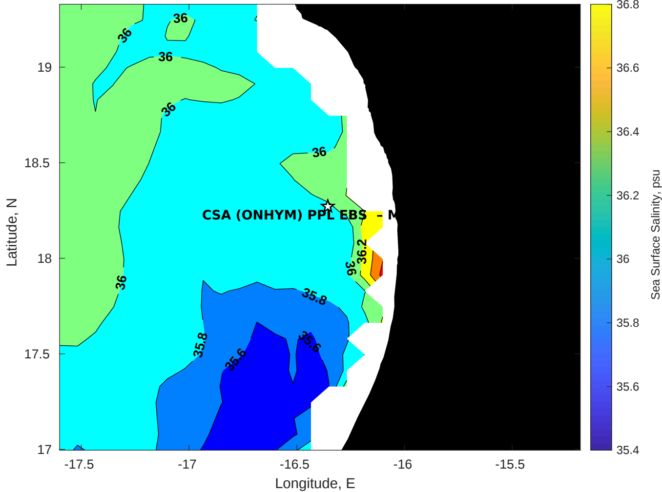
Surface Salinity for CSA (ONHYM) PPL EBS - Mauritania at 03-Nov-2025 00:00:00
