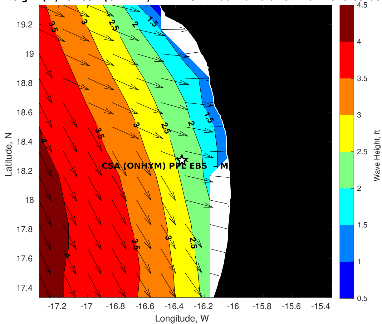
Wave Height (ft) for CSA (ONHYM) PPL EBS - Mauritania at 04-Nov-2025 09:00:00
