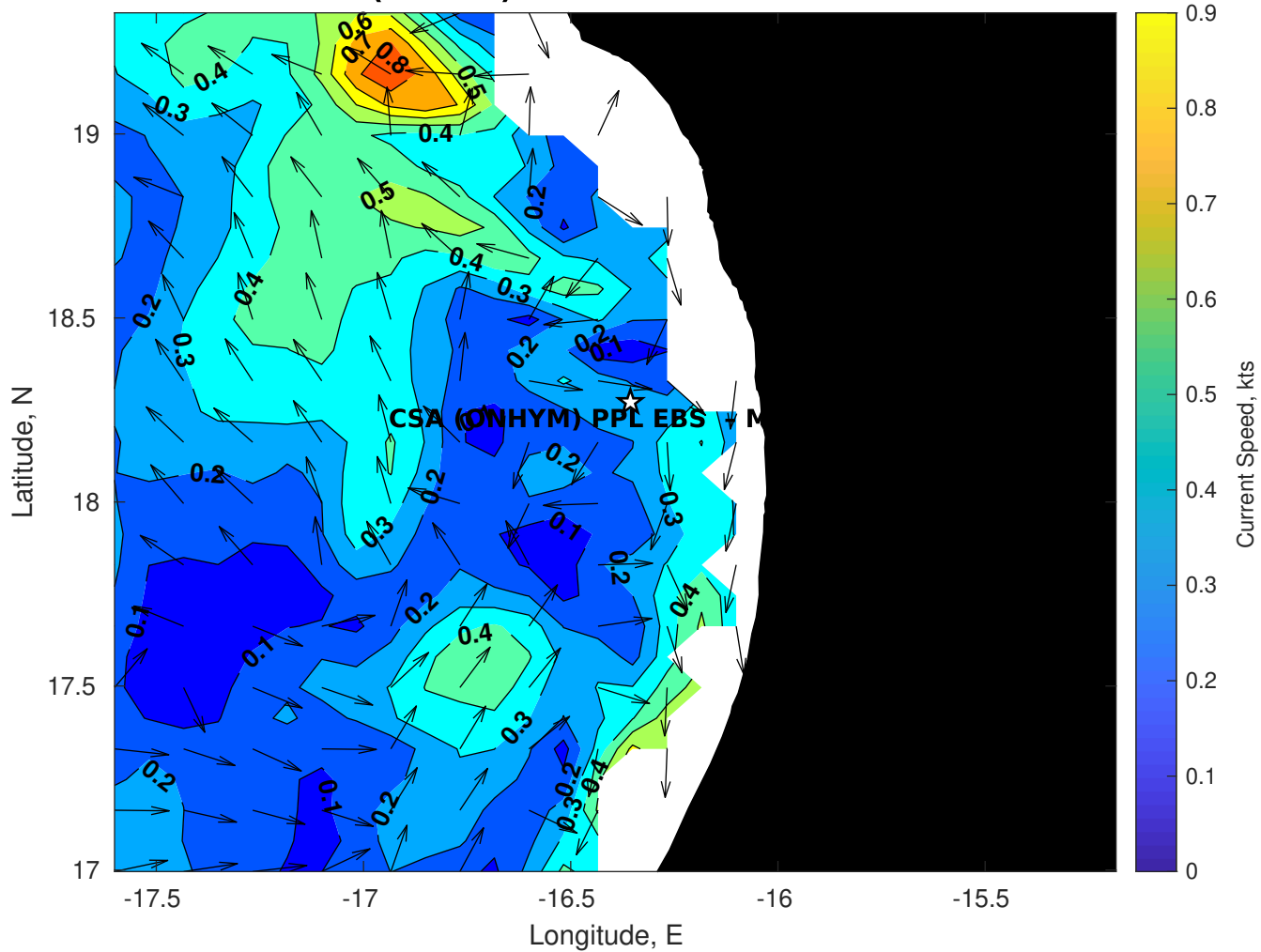
Surface Currents for CSA (ONHYM) PPL EBS - Mauritania at 03-Nov-2025 00:00:00
