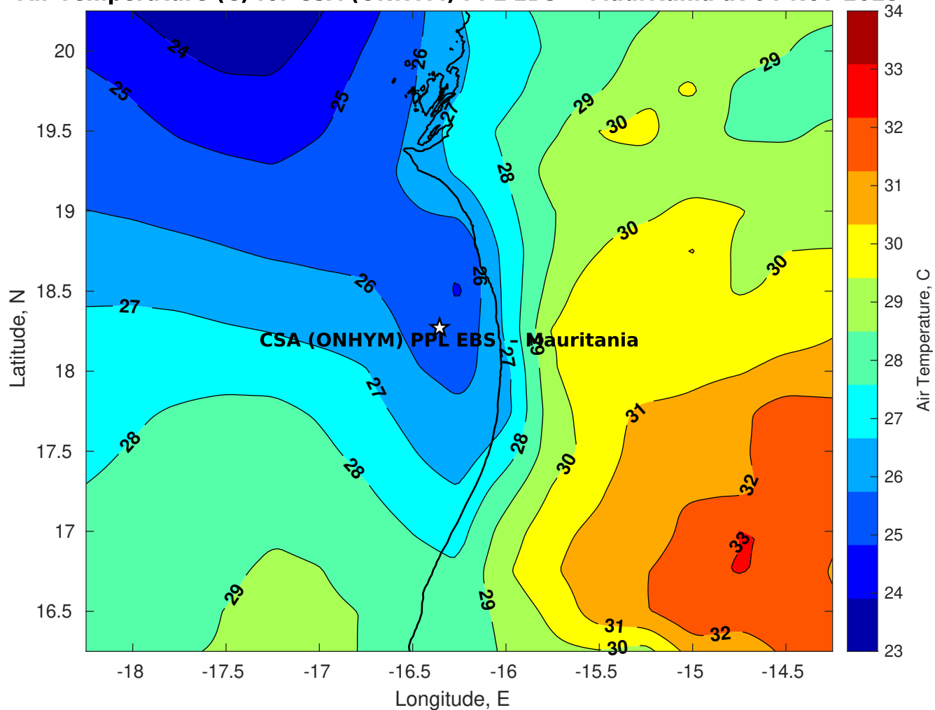
Air Temperature (C) for CSA (ONHYM) PPL EBS - Mauritania at 04-Nov-2025
