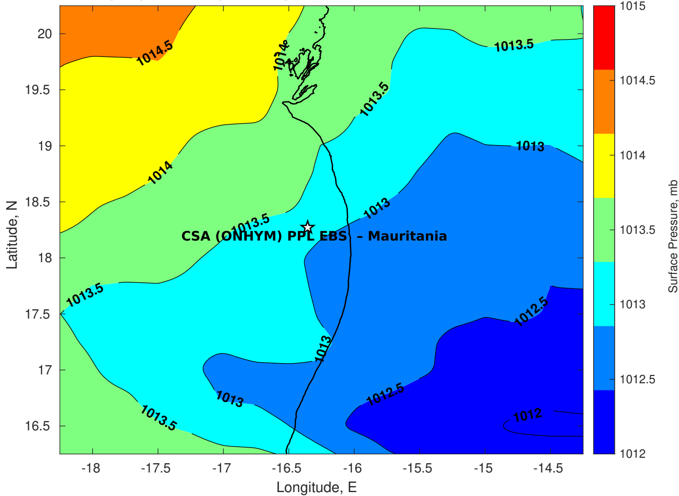
Surface Pressure (mb) for CSA (ONHYM) PPL EBS - Mauritania at 05-Nov-2025 00:00:00
