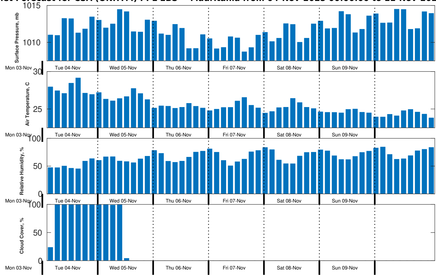
Met Forecast for CSA (ONHYM) PPL EBS - Mauritania from 04-Nov-2025 00:00:00 to 11-Nov-2025 00:00:00
