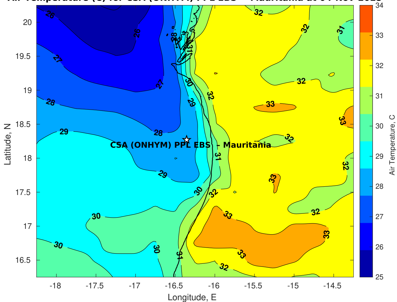
Air Temperature (C) for CSA (ONHYM) PPL EBS - Mauritania at 04-Nov-2025
