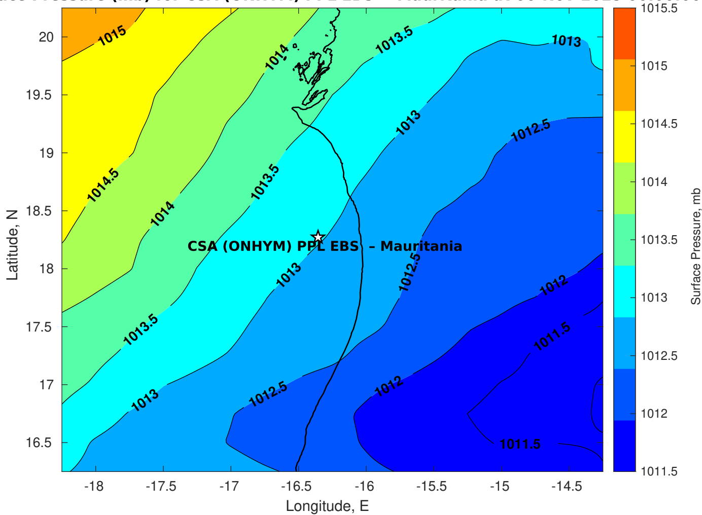
Surface Pressure (mb) for CSA (ONHYM) PPL EBS - Mauritania at 06-Nov-2025 00:00:00
