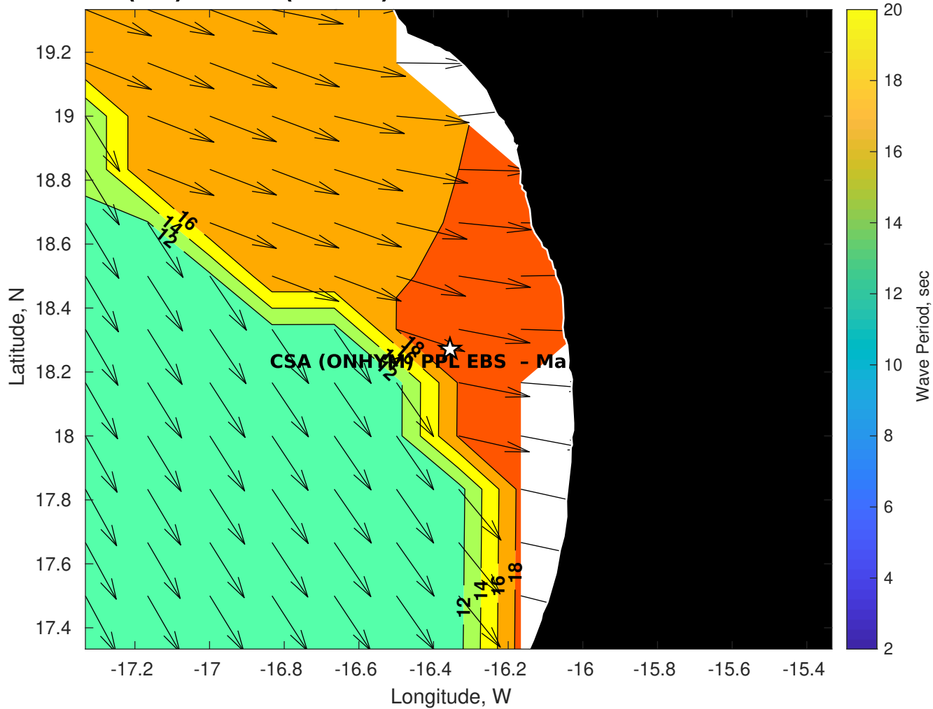
Wave Period (sec) for CSA (ONHYM) PPL EBS - Mauritania at 04-Nov-2025 09:00:00
