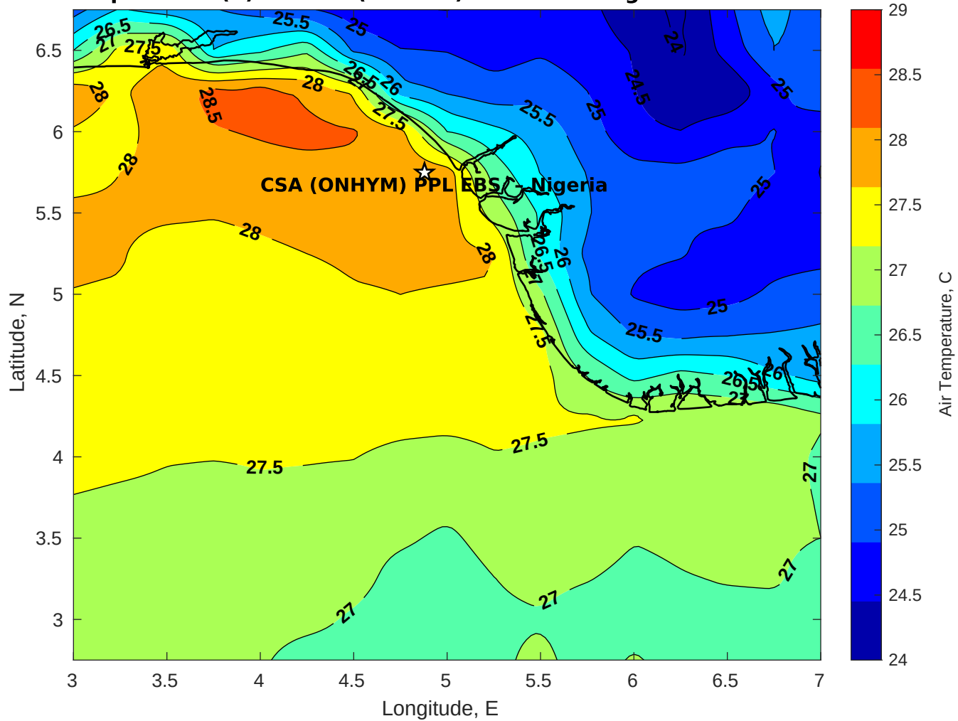
Air Temperature (C) for CSA (ONHYM) PPL EBS - Nigeria at 04-Nov-2025
