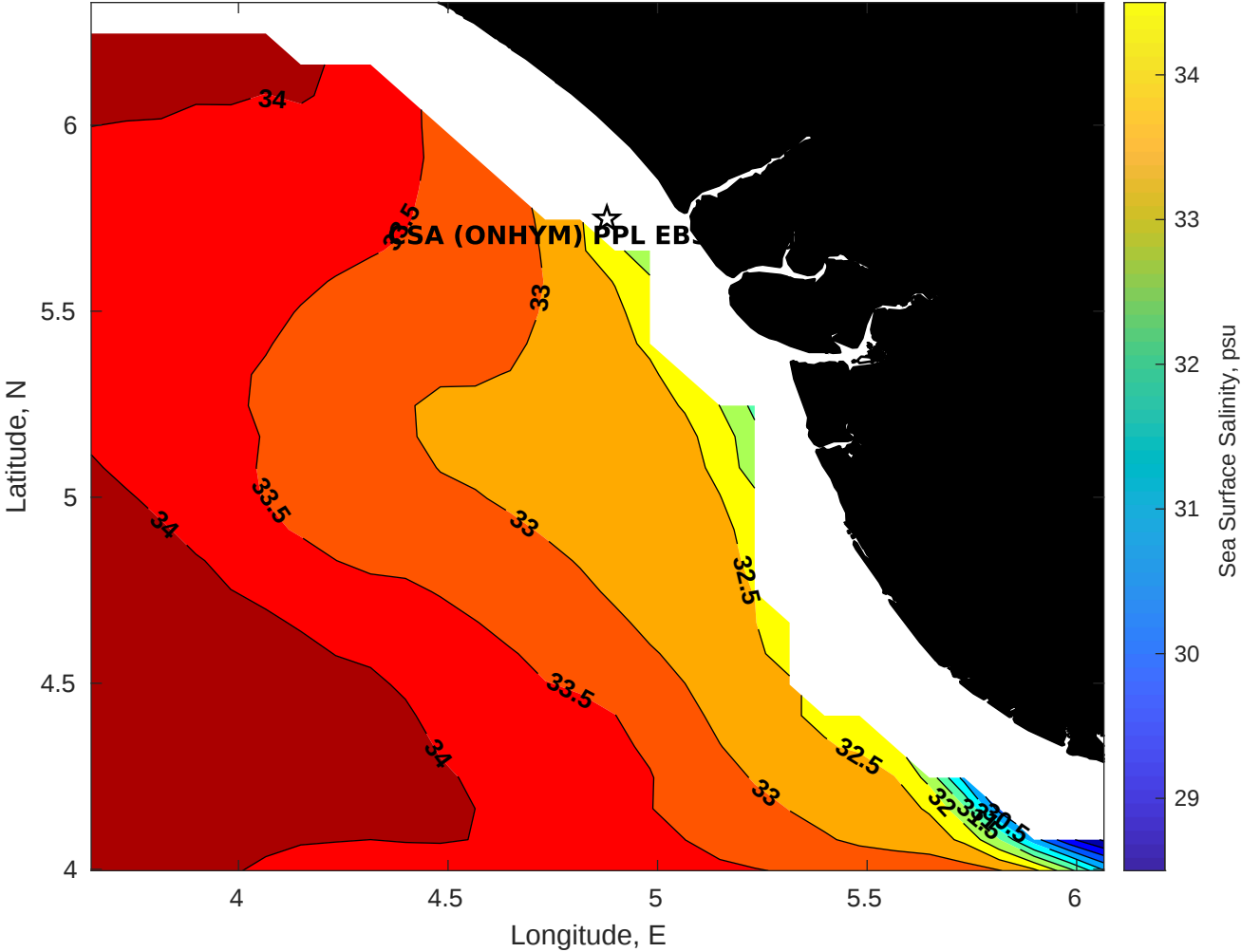
Surface Salinity for CSA (ONHYM) PPL EBS - Nigeria at 03-Nov-2025 00:00:00
